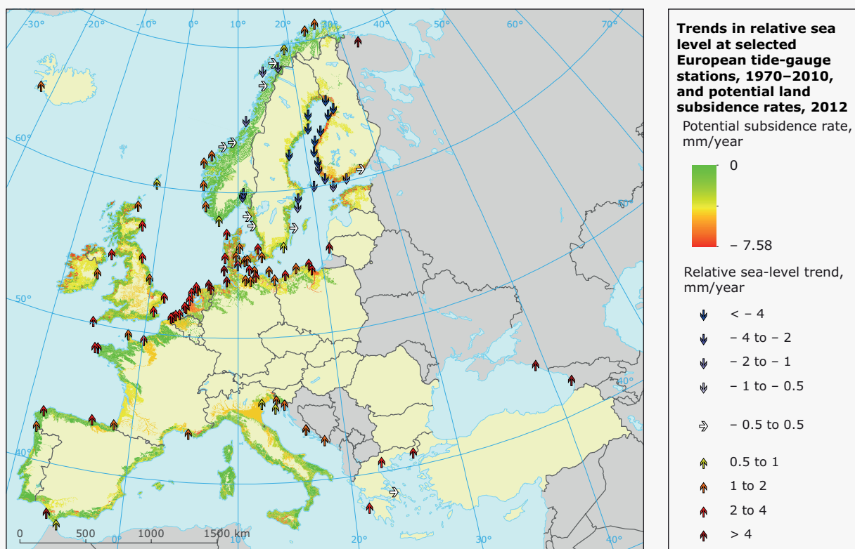
Map 3.2 Potential subsidence of coastal lowlands and relative sea-level trends in Europe
