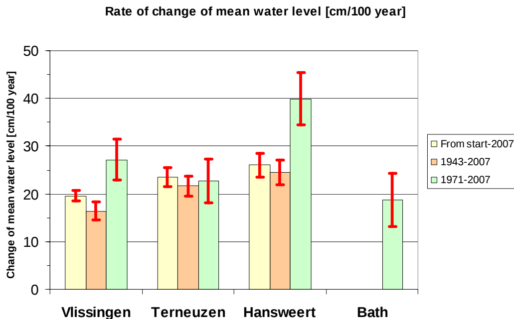
Figure 2.41: Slopes of linear regression lines and standard deviations for yearly-averaged mean water level in cm per 100 year. Note that the analysis periods for the four stations are different for the 'From start-2007' bars (depending on data availability).
