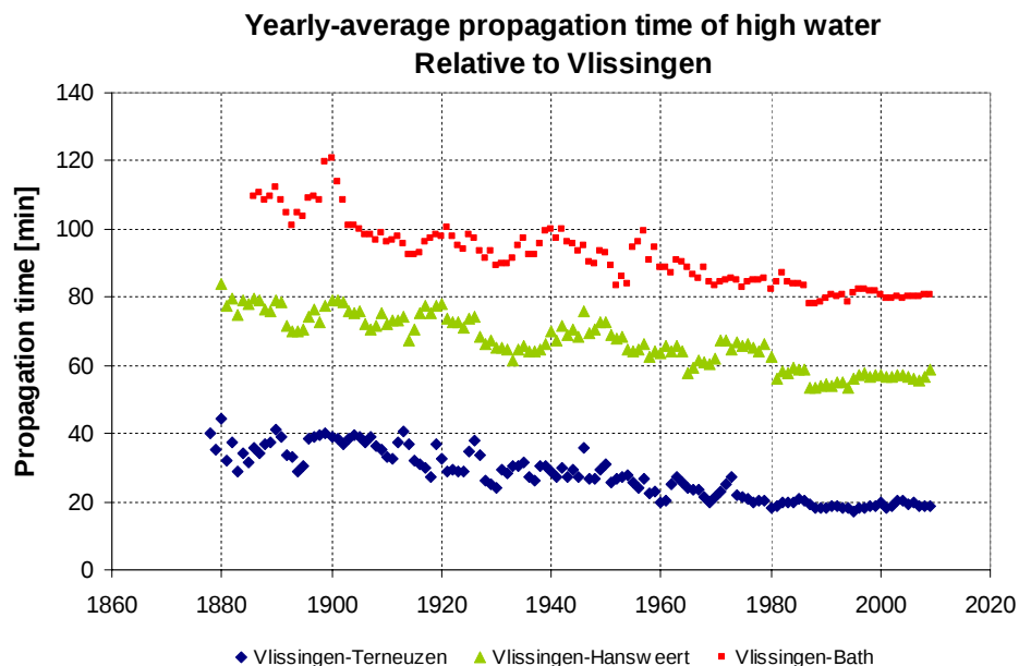
Figure 2.50: Yearly-averaged propagation time of high water in Terneuzen, Hansweert and Bath relative to Vlissingen.
