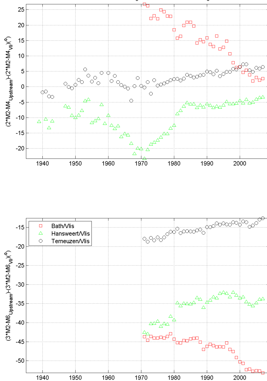
Figure A.16: Yearly M2, M4 and M6 tidal phase relationship ( 2 \cdot M2 - M4 and 3 \cdot M2 - M6 ) differences between upstream stations and Vlissingen
