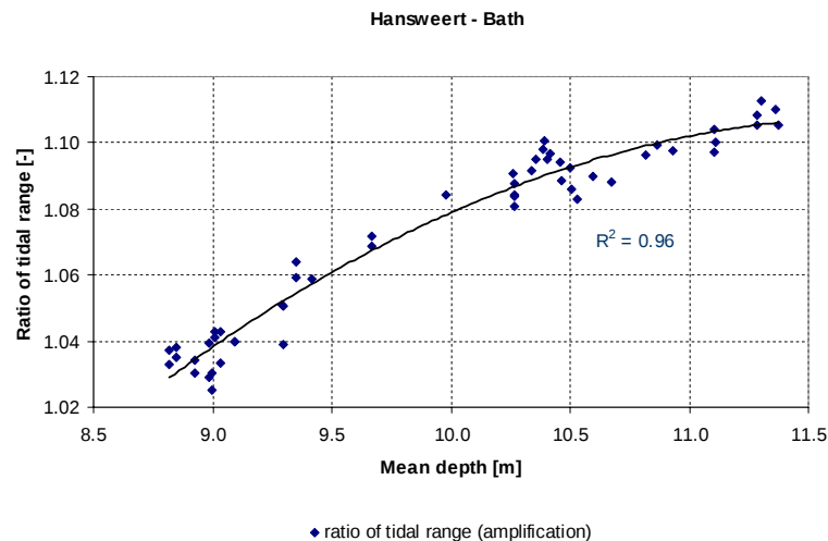
Figure 4.3: Ratio of tidal range (landward over seaward station) versus mean water depth for the section Hansweert-Bath approximated with a 2 nd order polynomial.
