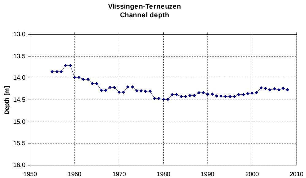
Figure 3.21: Channel depth for the section Vlissingen-Terneuzen.
