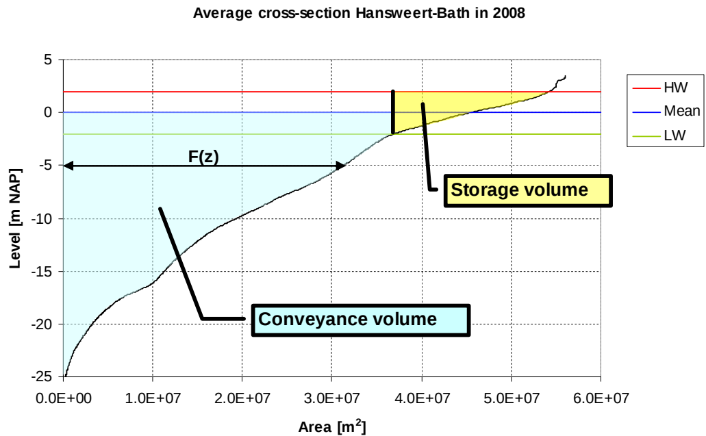
Figure 6.1: Hypsometric curve for the section Hansweert-Bath in 2008.
