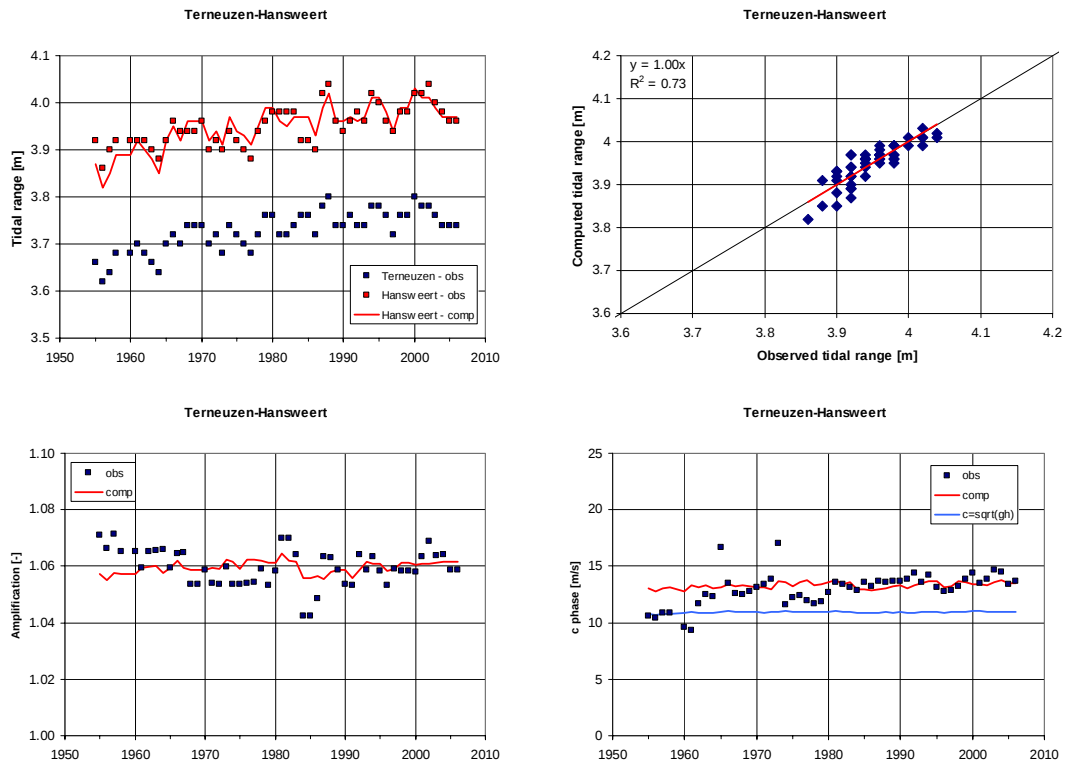
Figure 6.8: Observed 2^*M_2 -amplitude in Terneuzen and observed and computed 2^*M_2 -amplitude in Hansweert (upper left), regression observed and computed 2^*M_2 -amplitude in Hansweert (upper right), amplification of M_2 -amplitude in Hansweert (lower left) and observed and computed M_2 -phase velocity for the section Terneuzen-Hansweert (Ber9).
