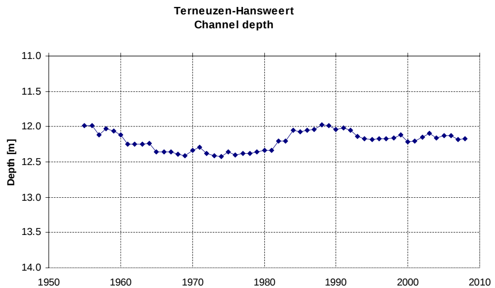
Figure 3.22: Channel depth for the section Terneuzen-Hansweert.
