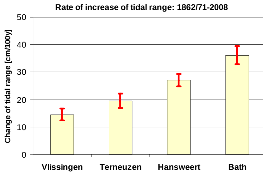
Figure C.6b: Rate of increase of tidal range in Vlissingen, Terneuzen, Hansweert and Bath as derived for the period 1862/1871 until 2008.
