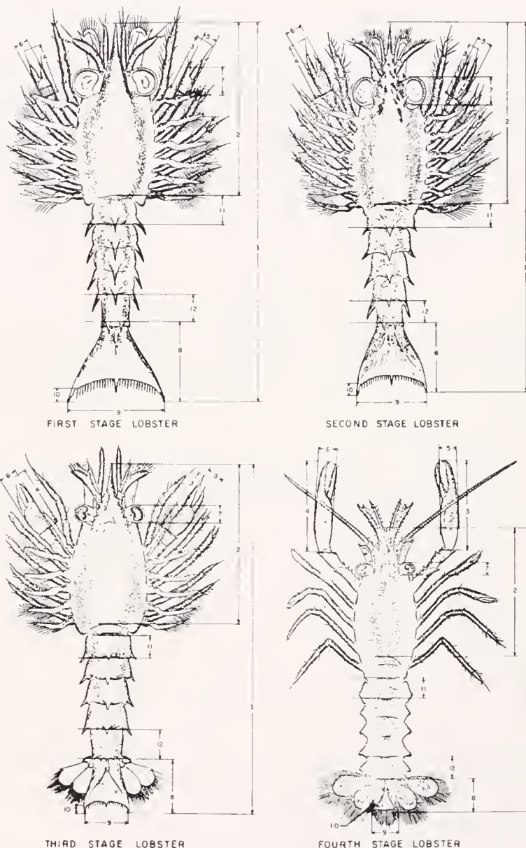
FIG. 2. Larval stages of the lobster, Homarus americanus (after Hadley, 1906). Numbers indicate characters measured. For the first, second and third stages the end of the segment just anterior to the telson was measured at the base of the spines since the true end of the segment was difficult to discern.
