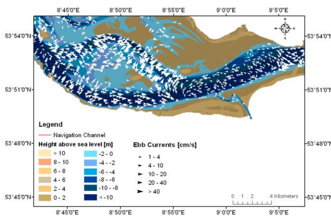
Figure 3. Differences in ebb currents [cm/s] between the reference scenario and the scenario 4 on October the 1 st of the year 2006 at 10 AM (Reference: Authors design).
