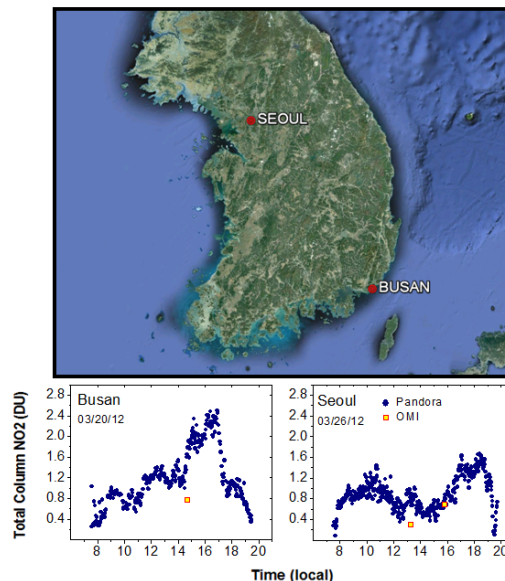
Figure 1 \text{TCNO}_2 variability in Seoul and Busan
