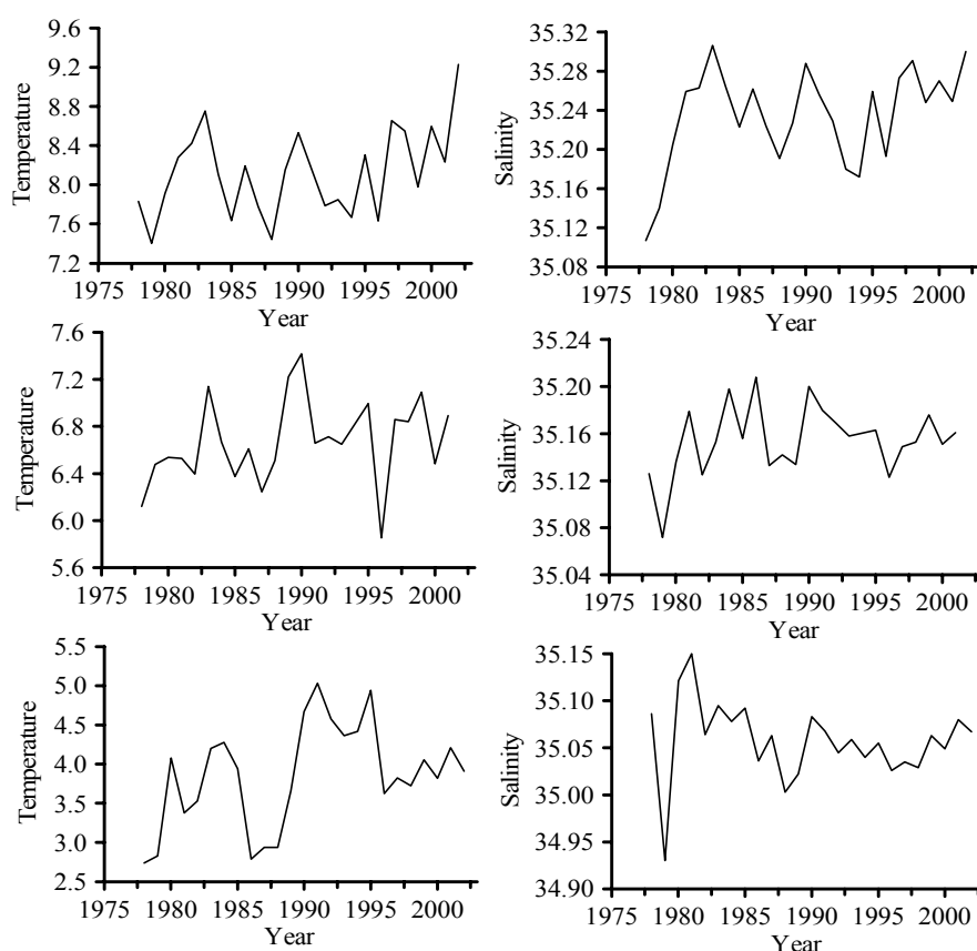
Figure 32. Area 10 – Norwegian Sea. Average temperature and salinity above the slope at three sections, Svinøy (approx. 63°N – upper figures), Gimsøy (approx. 69°N – central figures), and Sørkapp (approx. 76°N – lower figures), representing the southern, central, and northern Norwegian Sea.
