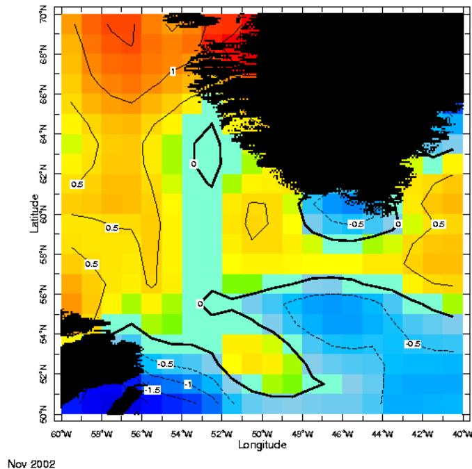
Figure 7. Area 1 – West Greenland. Sea surface temperature anomaly (K) off West Greenland during November 2002 (from: http://ingrid.lidgo.columbia.edu/SOURCES/IGOSS ).
