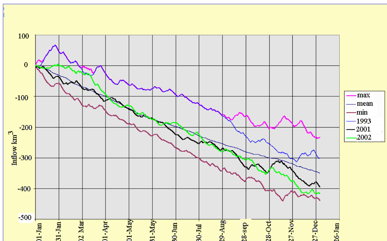
Figure 30. Area 9b – Skagerrak, Kattegat, and the Baltic. Accumulated inflow in km 3 through the Öresund in 1993, 2001, and 2002 compared with the period 1977–2001. The map was constructed by SMHI.
