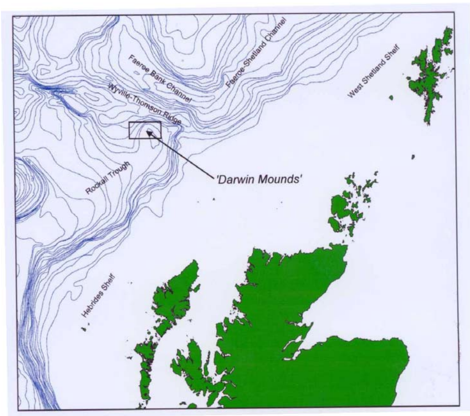
Figure 3.1.4.2. Location of Darwin Mounds in the Northeast Atlantic.
