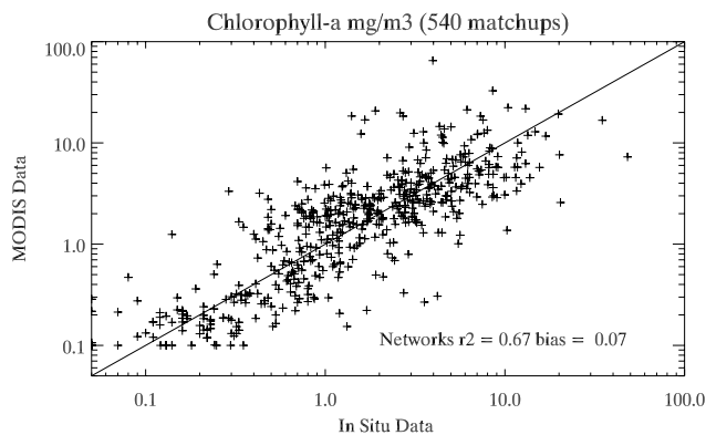
Fig. 2. MODIS-derived chlorophyll versus in-situ observations at the selected stations.
