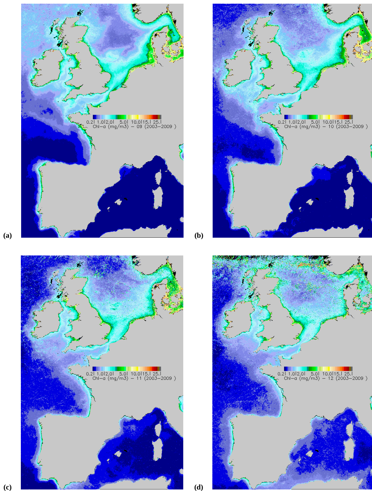
Fig. A3. Monthly chlorophyll- a concentration in September (a), October (b), November (c) and December (d).
