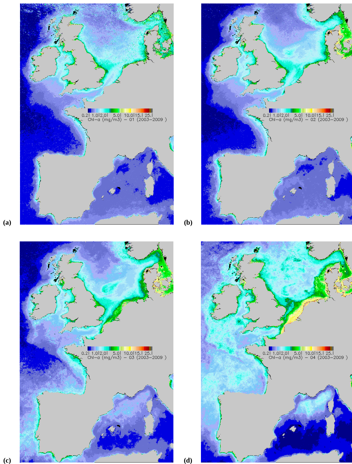
Fig. A1. Monthly chlorophyll- a concentration in January (a), February (b), March (c) and April (d).
