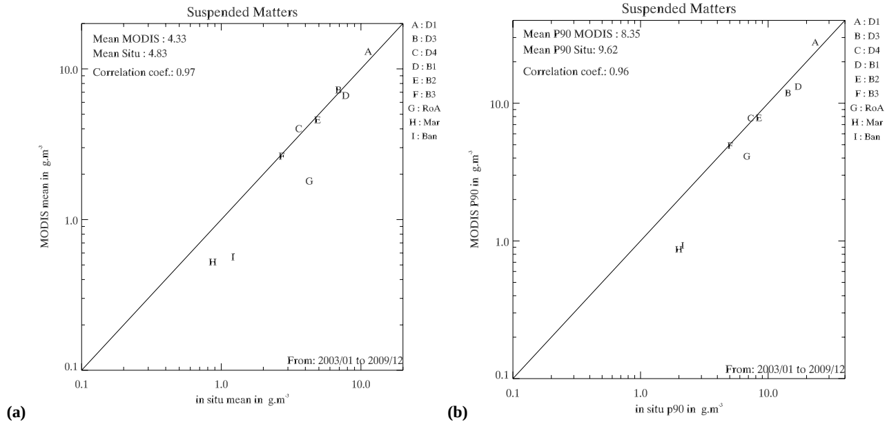
Fig. 8. Annual average (a) and P90 (b) of the MODIS and in-situ SPM.
