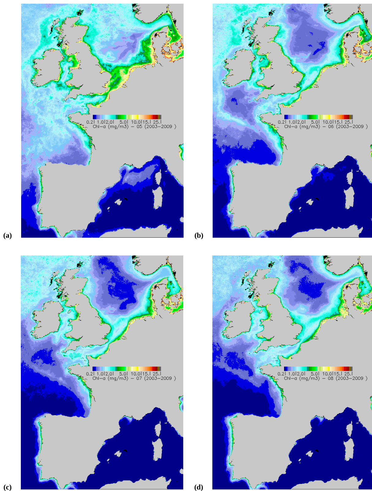
Fig. A2. Monthly chlorophyll- a concentration in May (a), June (b), July (c) and August (d).
