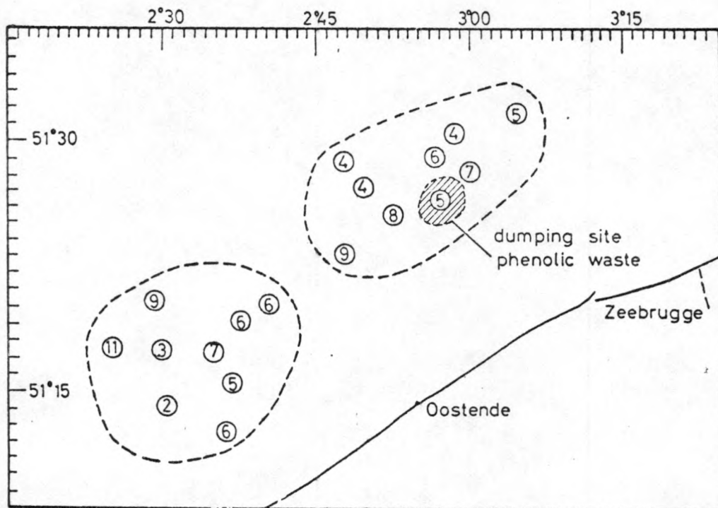
Fig. 1. — Western and Eastern sampling areas showing the average concentrations of phenolic compounds in the water (in ug/l).
