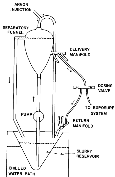
Figure 3. Sediment dosing system with chilled water bath and argon gas supply.
