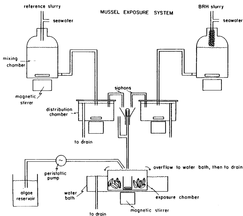
Figure 4. Exposure system used in the Black Rock Harbor experiments.
