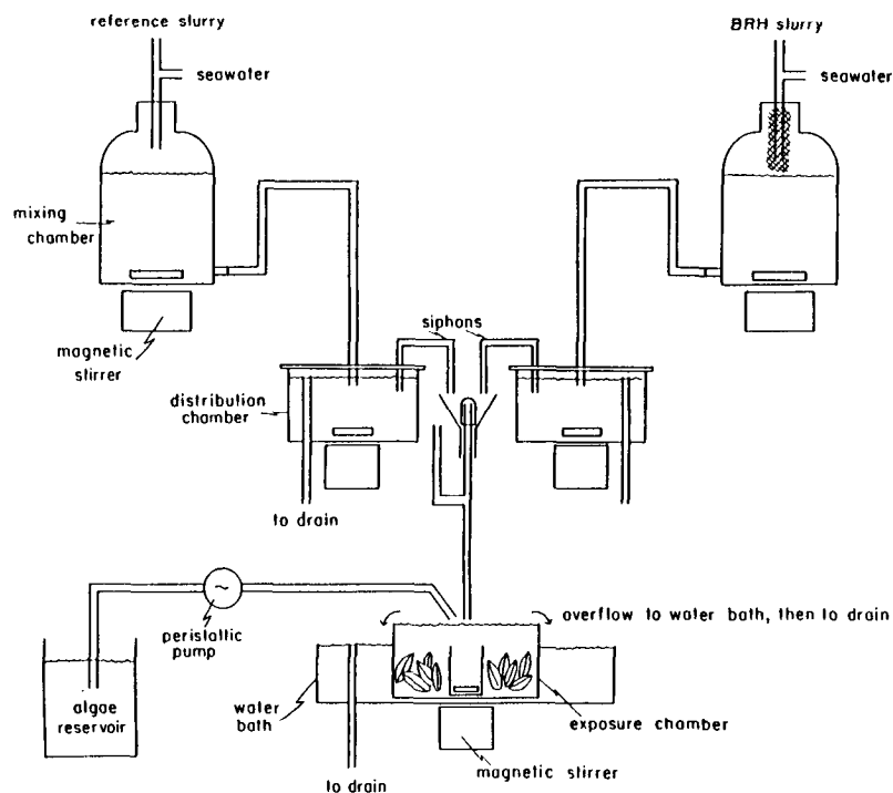
Figure 3. Schematic of the dosing system used to treat M. edulis with various concentrations of BRH and REF sediment suspensions
