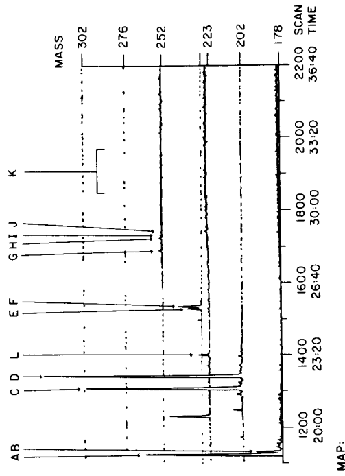
c. Filtrate
