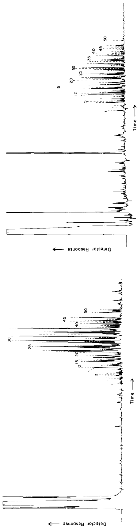
c. Filter
