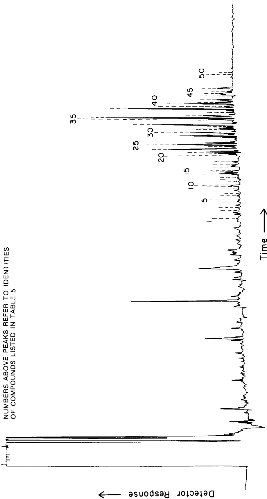
Figure 8. Capillary column electron capture gas chromatogram of PF-50 (PCB) fractions from mussel, time 0
