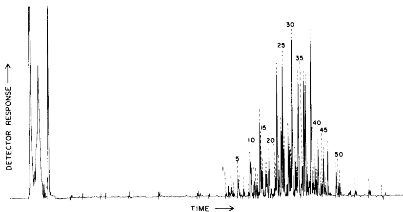
c. Day 28
