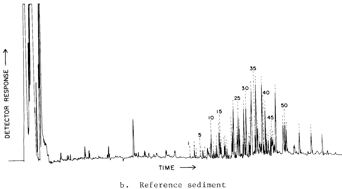
Figure 28. Capillary column electron capture gas chromatograms of PF-50 (PCB) fraction
