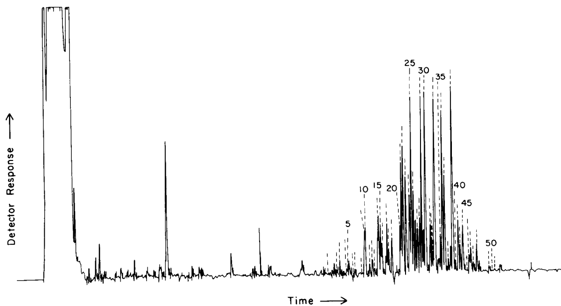
Figure 11. Capillary column electron capture gas chromatograms of PF-50 (PCB) fraction from exposure mussels
