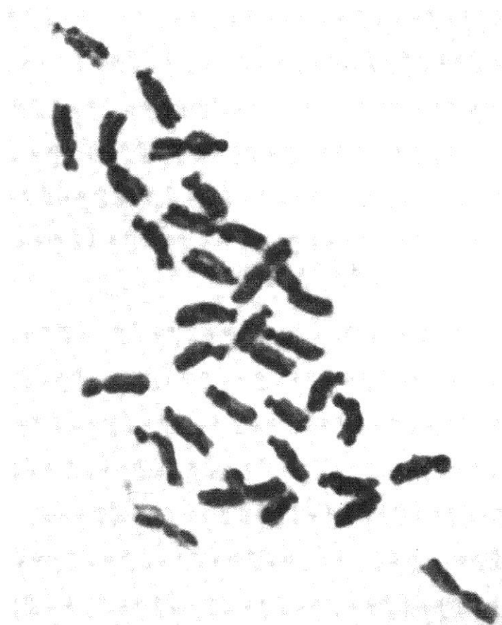
Figure 1. Sister chromatid exchange illustrated with the chromosomes of the polychaete N. incisa
