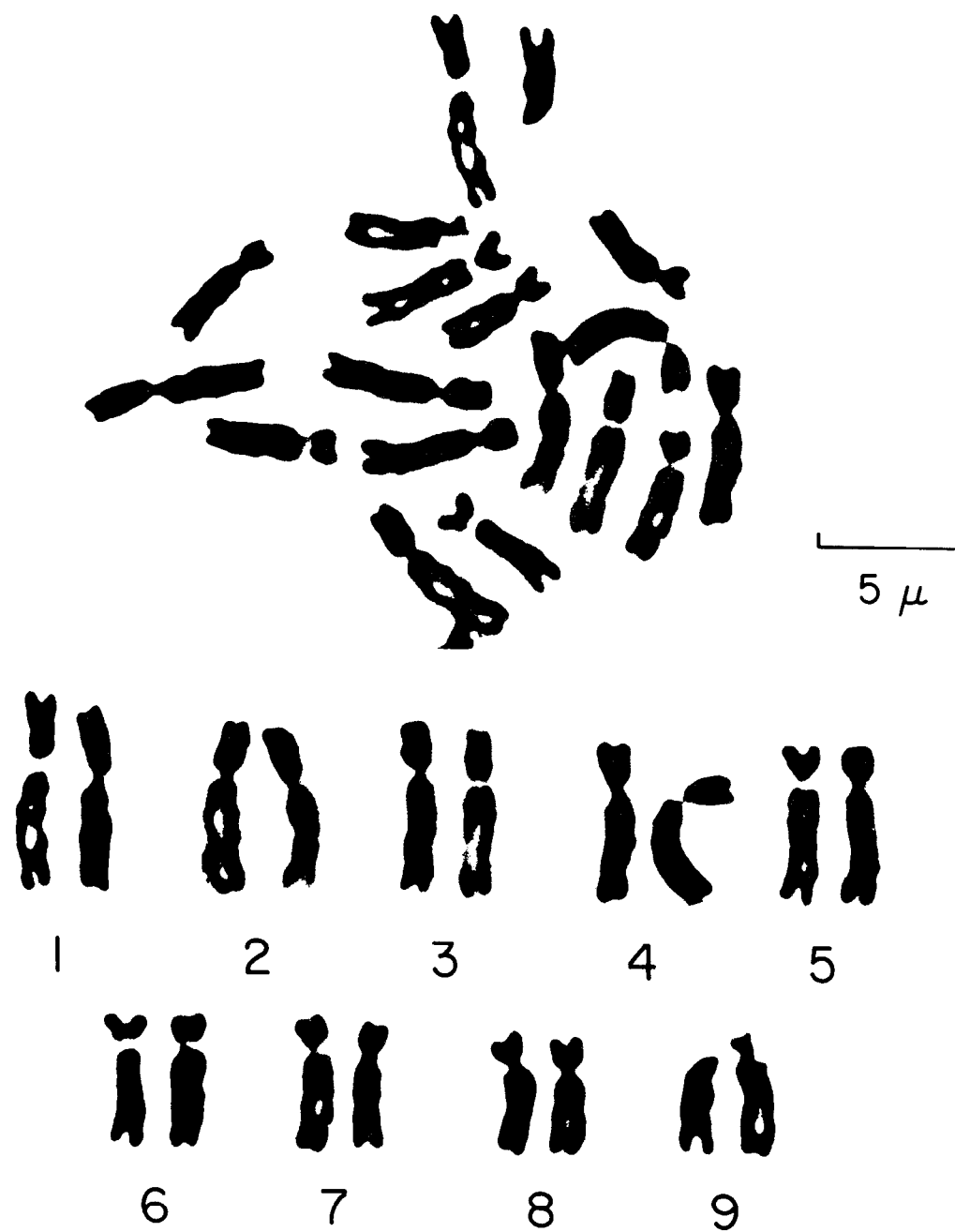
Figure A1. Chromosomes of Neanthes arenaceodentata
