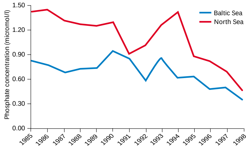
Figure 4 Change in average winter phosphate concentration in the Baltic Sea and the North Sea in the period 1985–98
