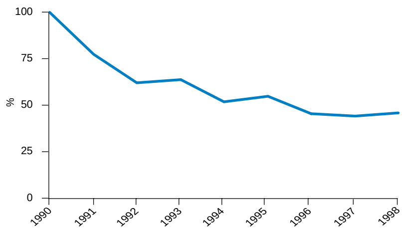
Figure 5 Index of loads (direct and riverine input) of hazardous substances into the North-East Atlantic including the North Sea in the period 1990–98 (index value in 1990 is 100 %. The index is the average of the yearly river concentrations of six hazardous substances)
