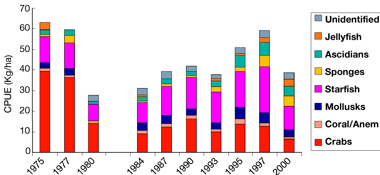
Fig. A4.5 Composition of invertebrate catch in selected bottom trawl surveys.
