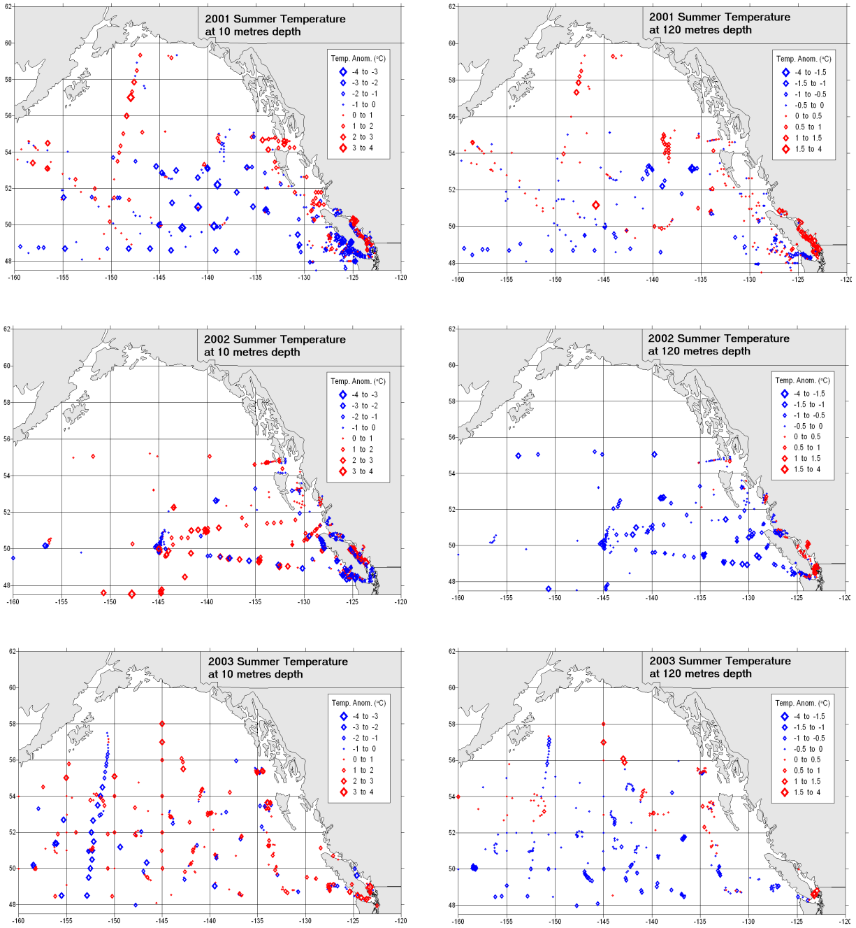
Fig. 1.16 Temperature anomalies (°C) at 10 and 120 m depth in the summers of 2001 to 2003. The size of the diamond represents the magnitude of the warm (red) or cold (blue) anomaly, according to the inset scale on each map. The near-surface waters were cooler than normal in 2001 in the southeast region and warmer in the northeast region. These anomalies weakened in the summer of 2002, and then reversed in 2003. Temperatures at 120 m depth show significant cooling in the southeast Gulf of Alaska in 2001 and 2002, with a weakening of this anomaly in 2003.
