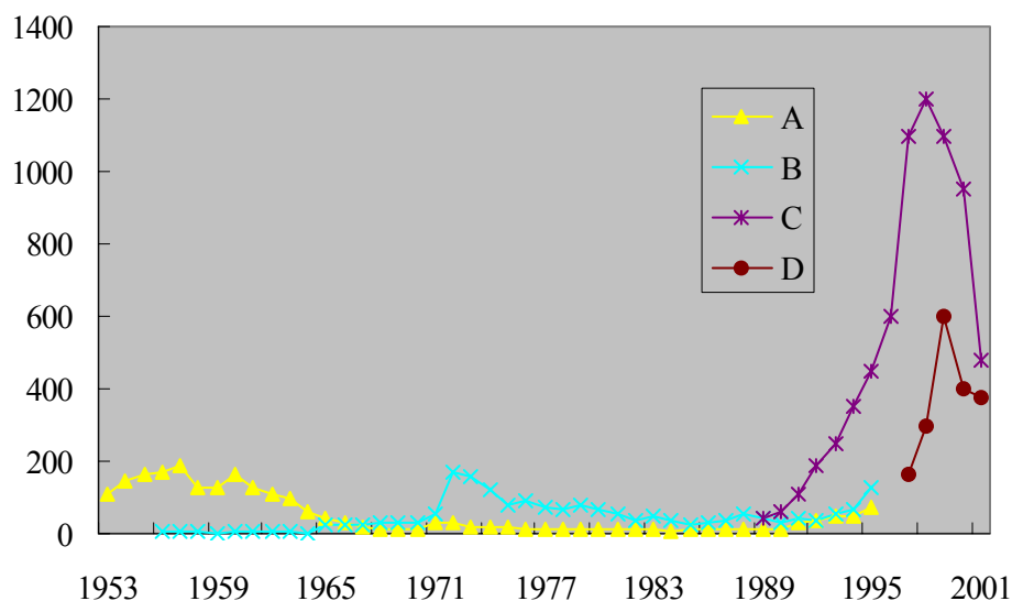
Fig. A5.13 Annual catch (tonnes) of dominant species in the Yellow Sea: (A) small yellow croaker and hairtail, (B) Pacific herring and Japanese mackerel, (C) anchovy, and (D) sandlance (adapted from Tang 2003).
