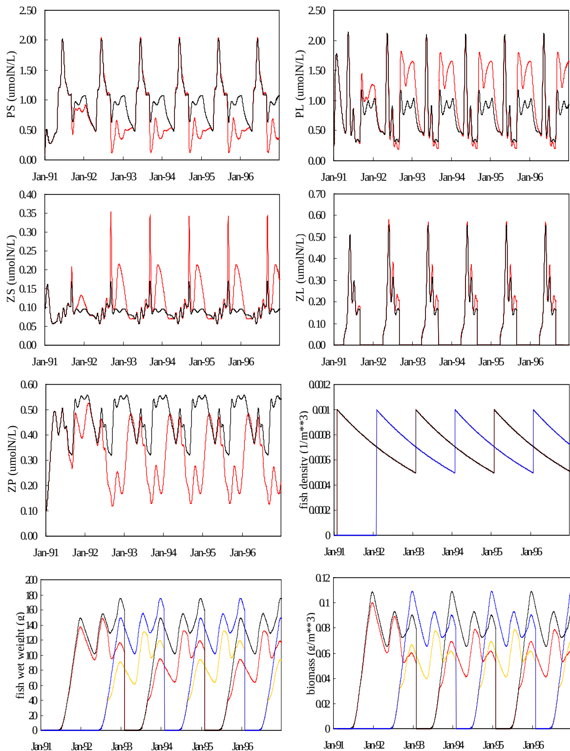
Fig. 2.5 Phytoplankton (PS, PL) and zooplankton (ZS, ZL, ZP) density and numbers, wet weight, biomass of saury calculated by NEMURO.FISH with two overlapping cohorts, saury (red: two-way first cohort, orange: two-way second cohort, black: one-way first cohort, blue: one-way second cohort).
