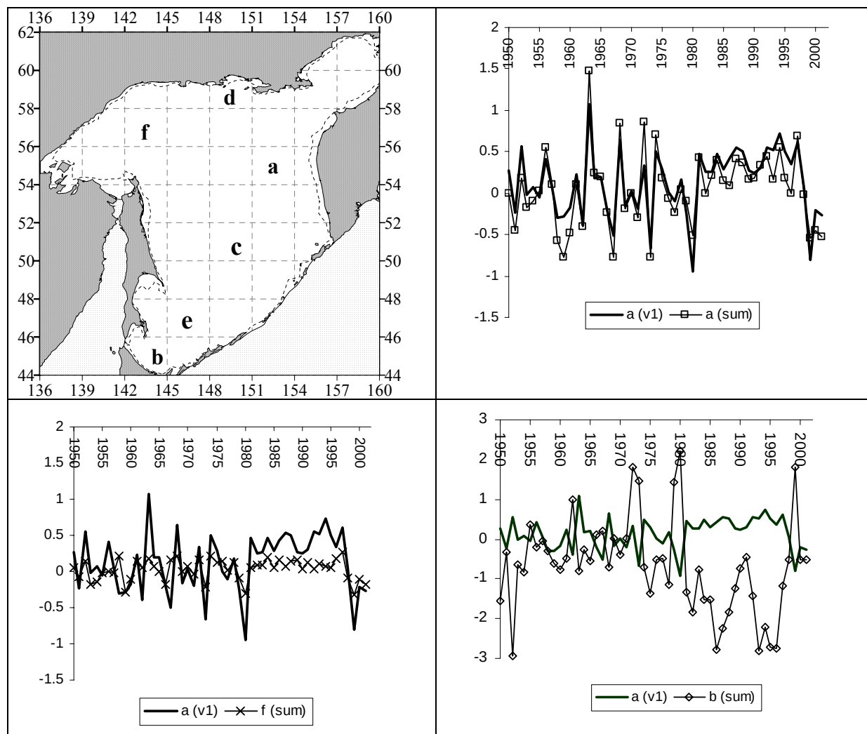
Fig. 2 Interannual variability of contribution of the first EOF component only (bold) and the sum of the first four components (light) at the horizon of 50 m (°C) for the different squares of the Okhotsk Sea.
