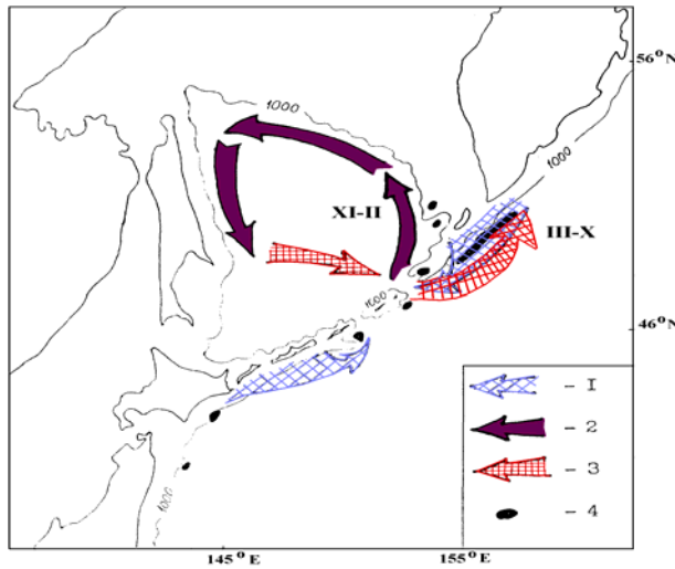
Fig. 2 The scheme of horizontal migrations of the giant grenadier along the Kuril Islands and in the Okhotsk Sea. 1- autumn-winter migrations of adult fish along the slope of Kuril Islands. 2- drifts of fish eggs and larvae. 3- spawning migration of adult fish. 4- concentrations of adult fish.
