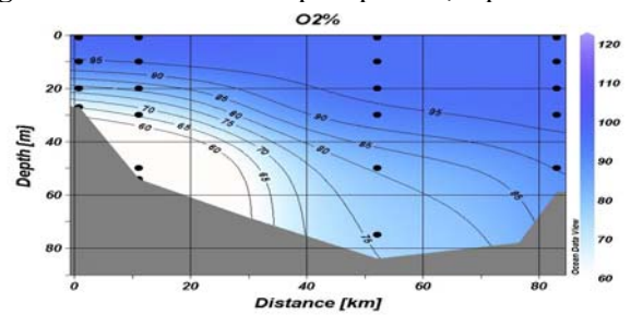
Fig. 9 Distribution of oxygen, section 3, August 2002.
