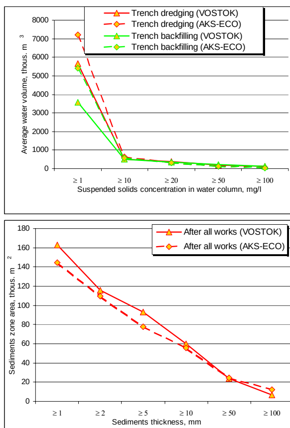
Fig. 1 Example of comparative diagrams on modeling results: (a) average contaminated water volumes during trenching and backfilling (total works volume – 800,000 m 3 ), (b) area of sediments formed on the sea bottom during site leveling (total works volume – 5,000 m 3 ).
