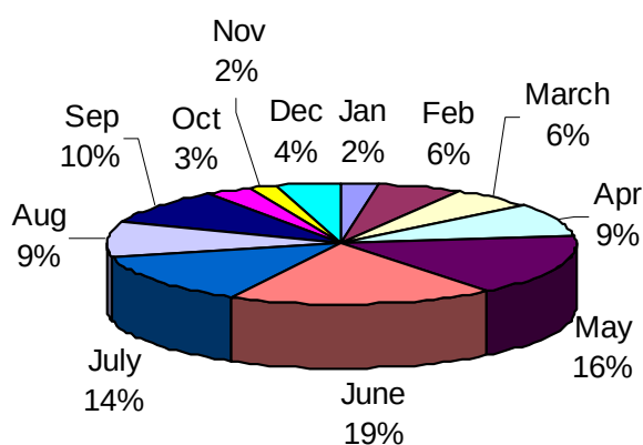
Fig. 7 The contribution of flatfishes by months averaged from 1999 to 2001(%).
