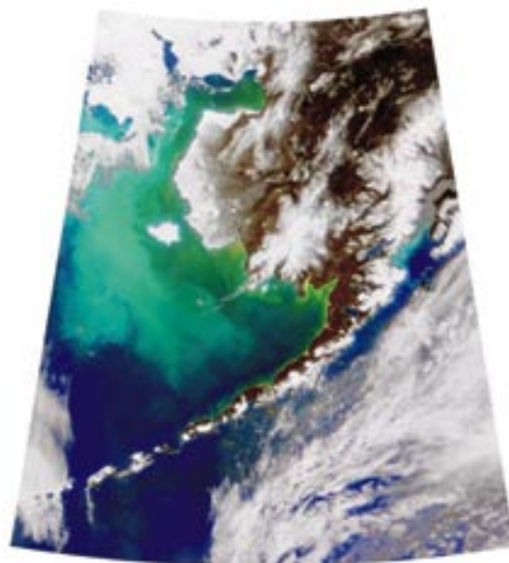
[Figure 5] A coccolithophore bloom (milky green waters) in the Bering Sea on April 25, 1998. 6
