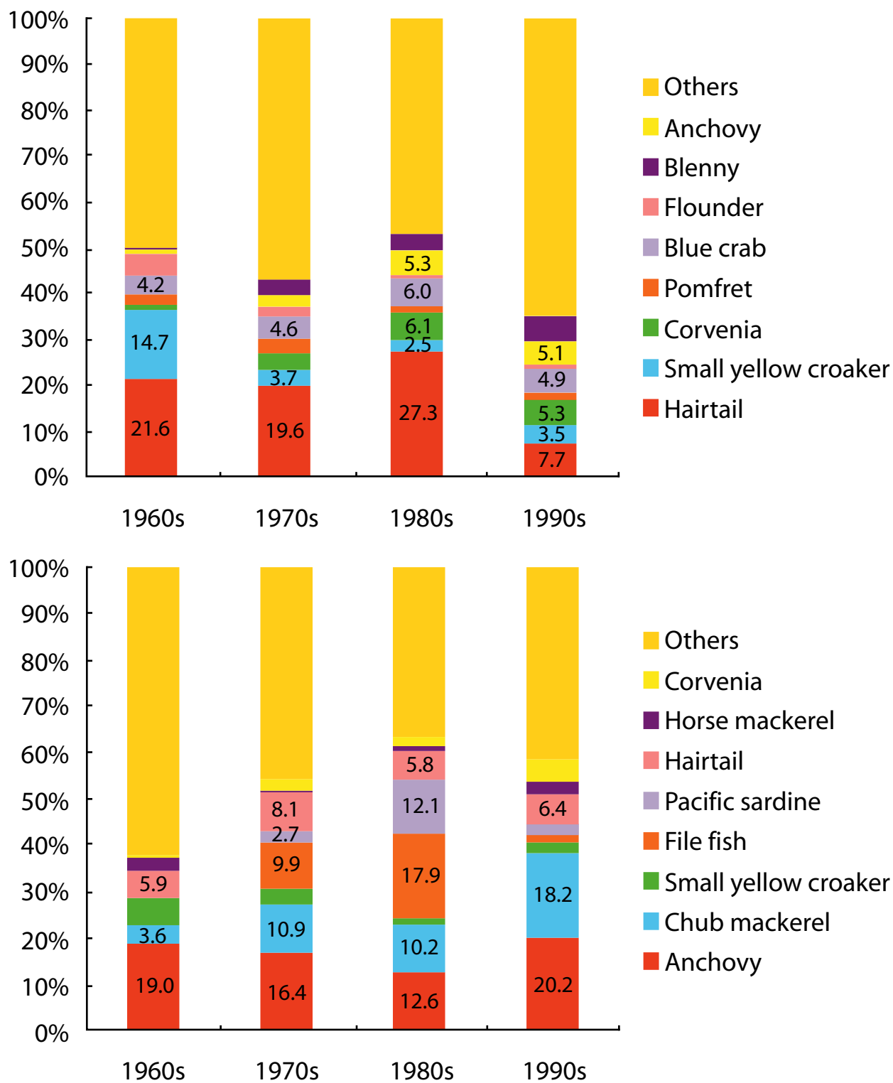
[Figure 9] Catch percentages by species (1961-2000) in the Yellow Sea (upper) and East China Sea (lower). 9
