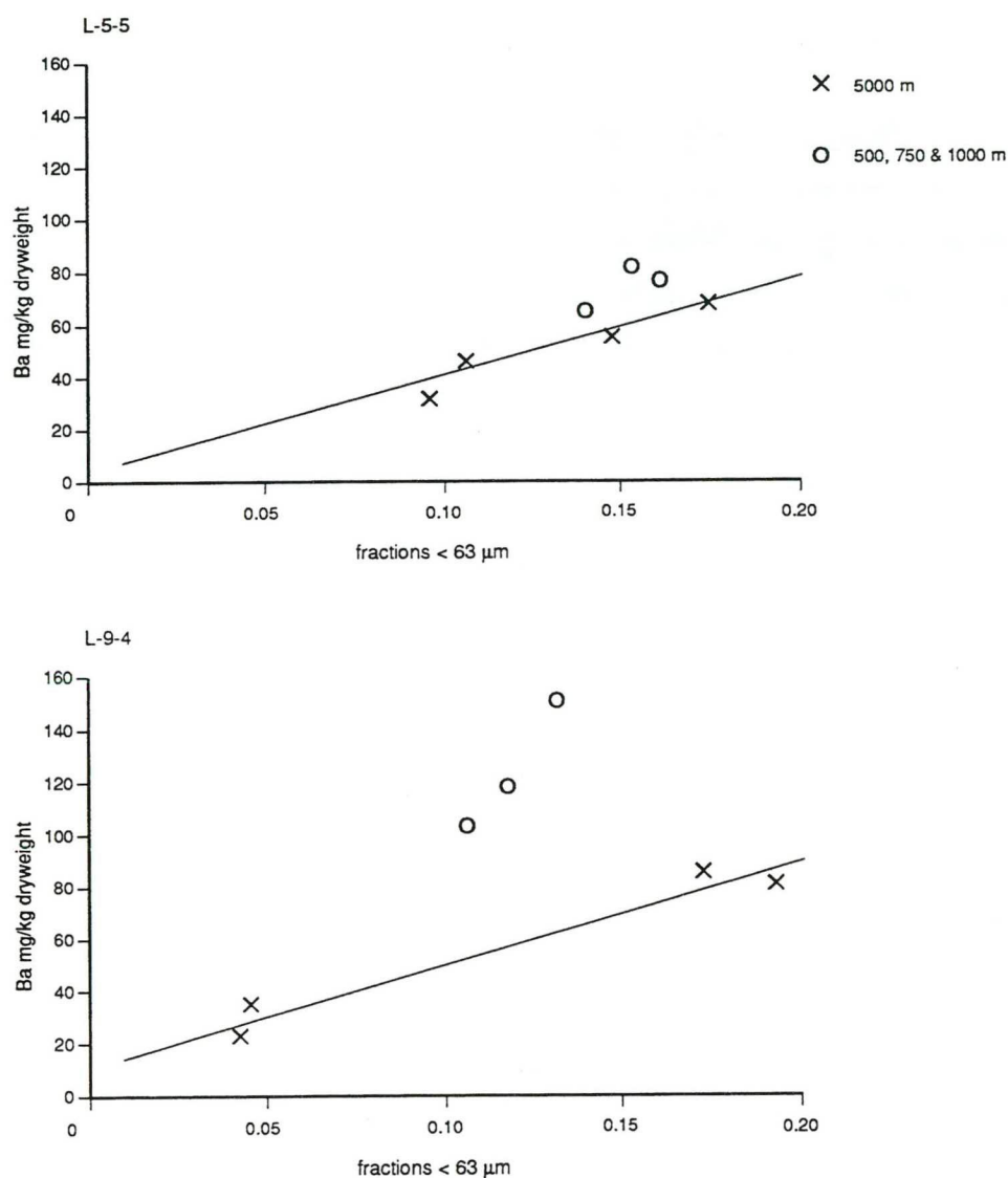
Fig. 6. The correlation between the barium content and the fraction < 63 \mu m of sediments at reference stations (5000m; background level = regression line), compared to those at stations 500-1000m from the drilling locations L-5-5 (above) and L-9-4 (below).
