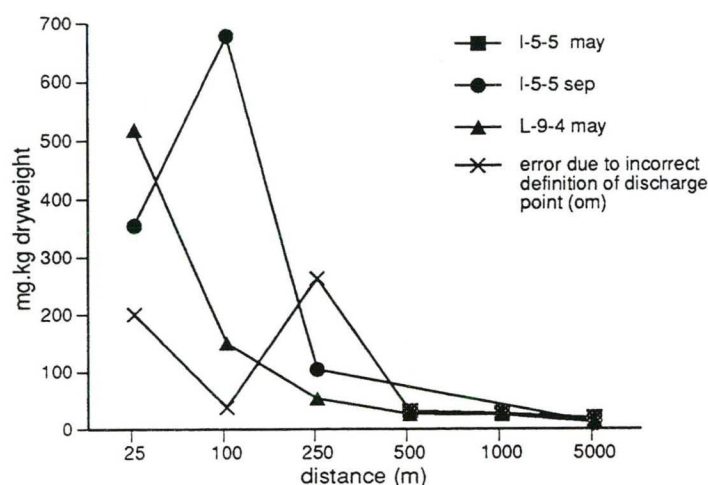
Figure 8: “Total” oil content of sediments (expressed on the basis of total dry weight) along a transect in the residual current direction at locations L-9-4 (May) and L-5-5 (May and September).
