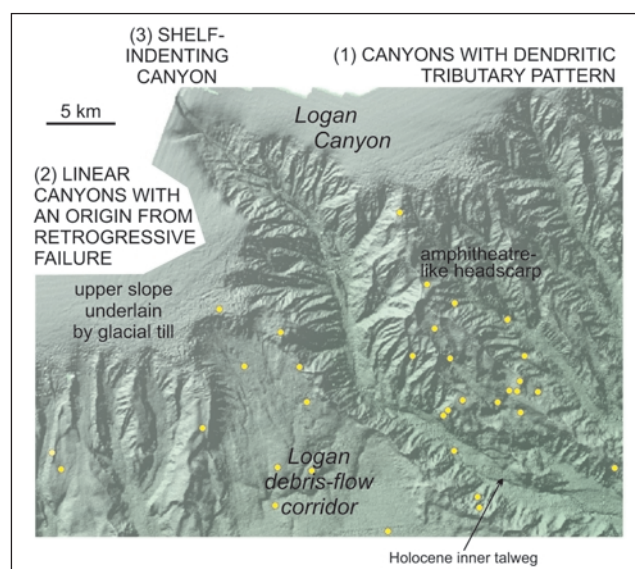
Figure 5. Multibeam bathymetry on the central Scotian Slope showing different types of canyons. 1 = dendritic canyons, just down-flow from The Gully outlet (Fig. 2); 2 = more linear retrogressive canyons; 3 = Logan Canyon, a large canyon cutting the shelf break with a Holocene inner talweg. Image modified from Mosher et al. (2004).
