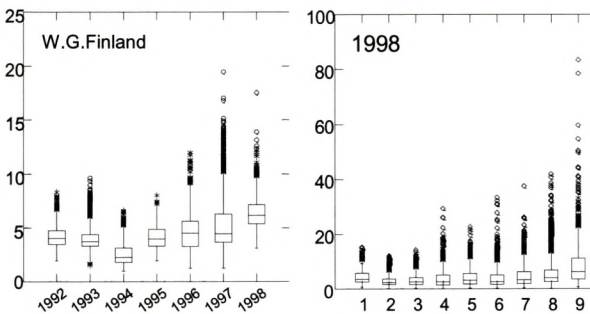
Figure 6. Left: annual variation in the summer concentrations of chlorophyll a (mg m -3 ) in the Gulf of Finland. Right: Regional variation in the spring concentrations of chlorophyll a (mg m -3 ) in the Baltic Sea (1= Travemünde, 2= Mecklenburg Bight, 3= Arkona Sea, 4= Western Bornholm Sea, 5= Northern Bornholm Sea, 6= Western Gotland Sea, 7= Eastern Gotland Sea, 8= Northern Baltic Proper and 9= Western Gulf of Finland)
