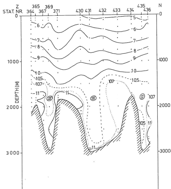
Fig. 13. The distribution of dissolved silicate ( \mu\text{M} ) in the vertical crosssection IV (cf. Fig. 5).
