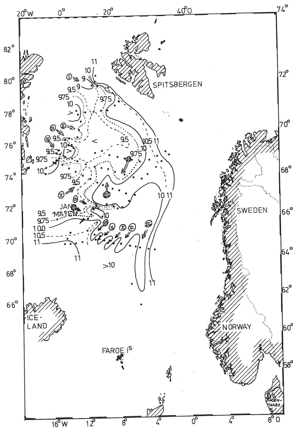
Fig. 8. A horizontal crosssection through the investigated area on a depth of 1250 meter, showing the distribution of dissolved silicate ( \mu\text{M} ).
