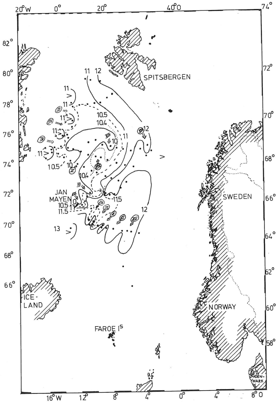
Fig. 9. A horizontal crosssection through the investigated area on a depth of 2000 meter, showing the distribution of dissolved silicate ( \mu\text{M} ).
