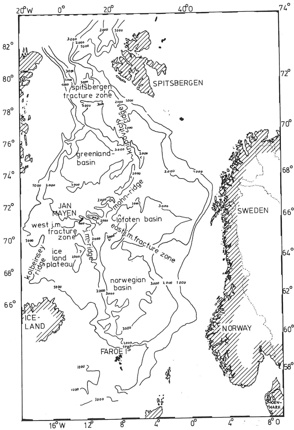
Fig. 1. Simplified bathymetry and names of the ridges and basins in the investigated area.
