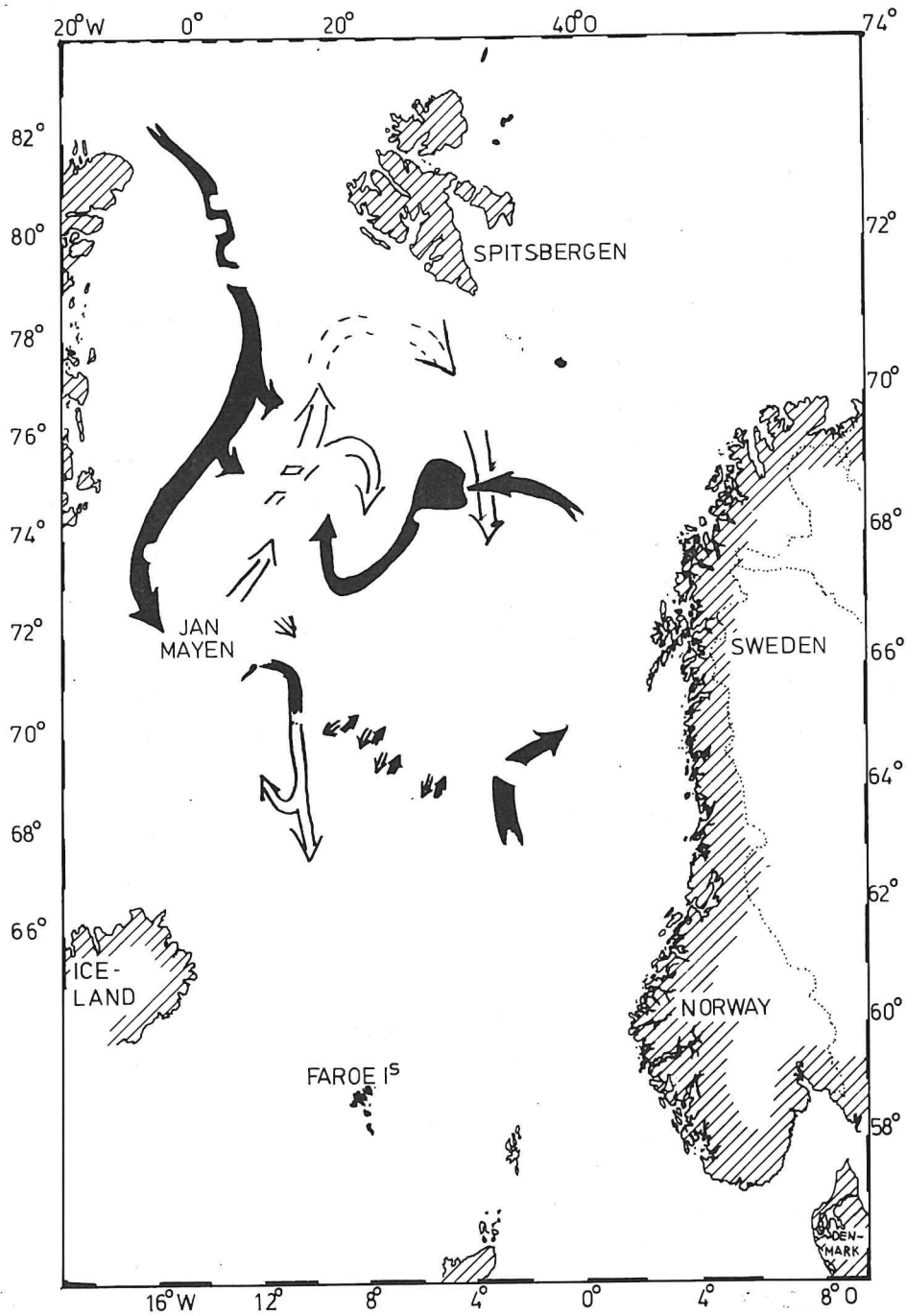
Fig. 20. A possible circulation-pattern based on horizontal gradients of dissolved silicate. White arrows point in the direction of an increasing silicate-concentration, dark arrows in the direction of decreasing silicate-concentrations.
