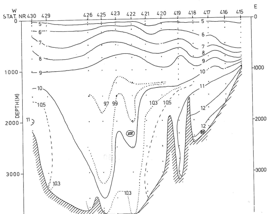
Fig. 11. The distribution of dissolved silicate ( \mu\text{M} ) in the vertical crosssection III (cf. Fig. 5).
