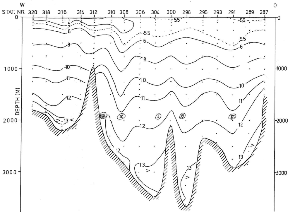
Fig. 10. The distribution of dissolved silicate ( \mu\text{M} ) in the vertical crosssection I (cf. Fig. 5).
