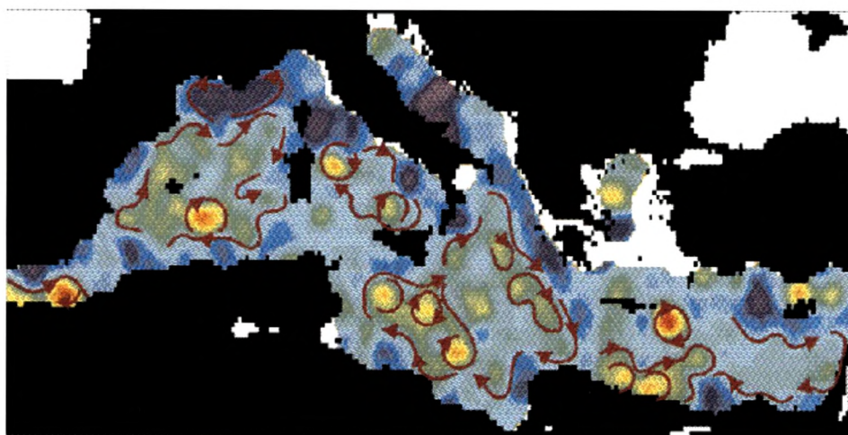
Figure 17: Analysis of Sea Surface Height anomaly from satellite altimetry
