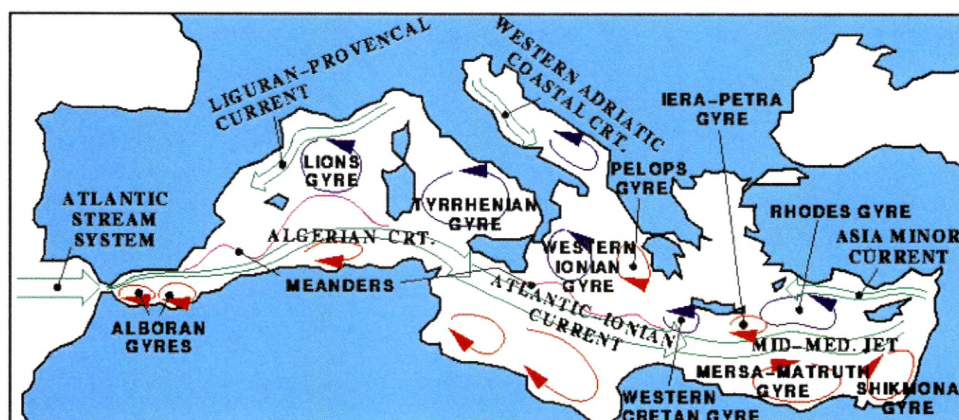
Figure 10b: Schematic of Mediterranean Sea general circulation. Structures from both observations and model results.
