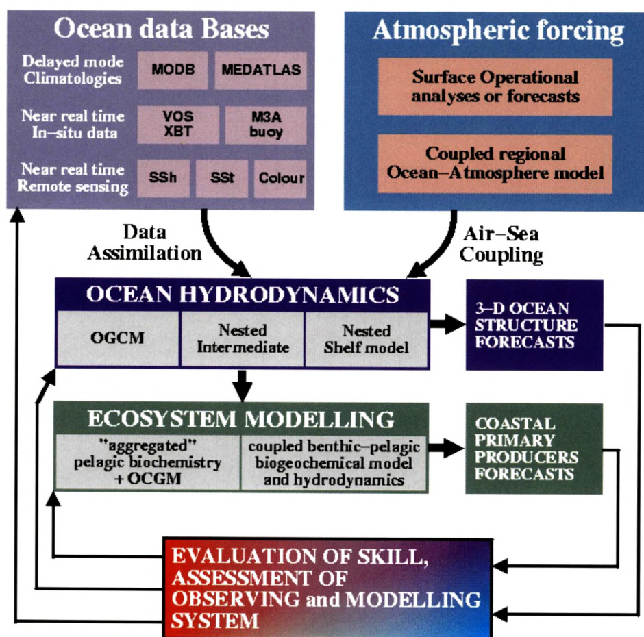
Figure 19. Schematic of the MFSPP methods and tools
