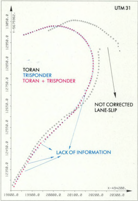
fig. 11 : radio equipment and the navigation systems Toran and Trisponder (above left) fig. 12 : XY - plot of test track with lane-slip and small drift. (above right)
