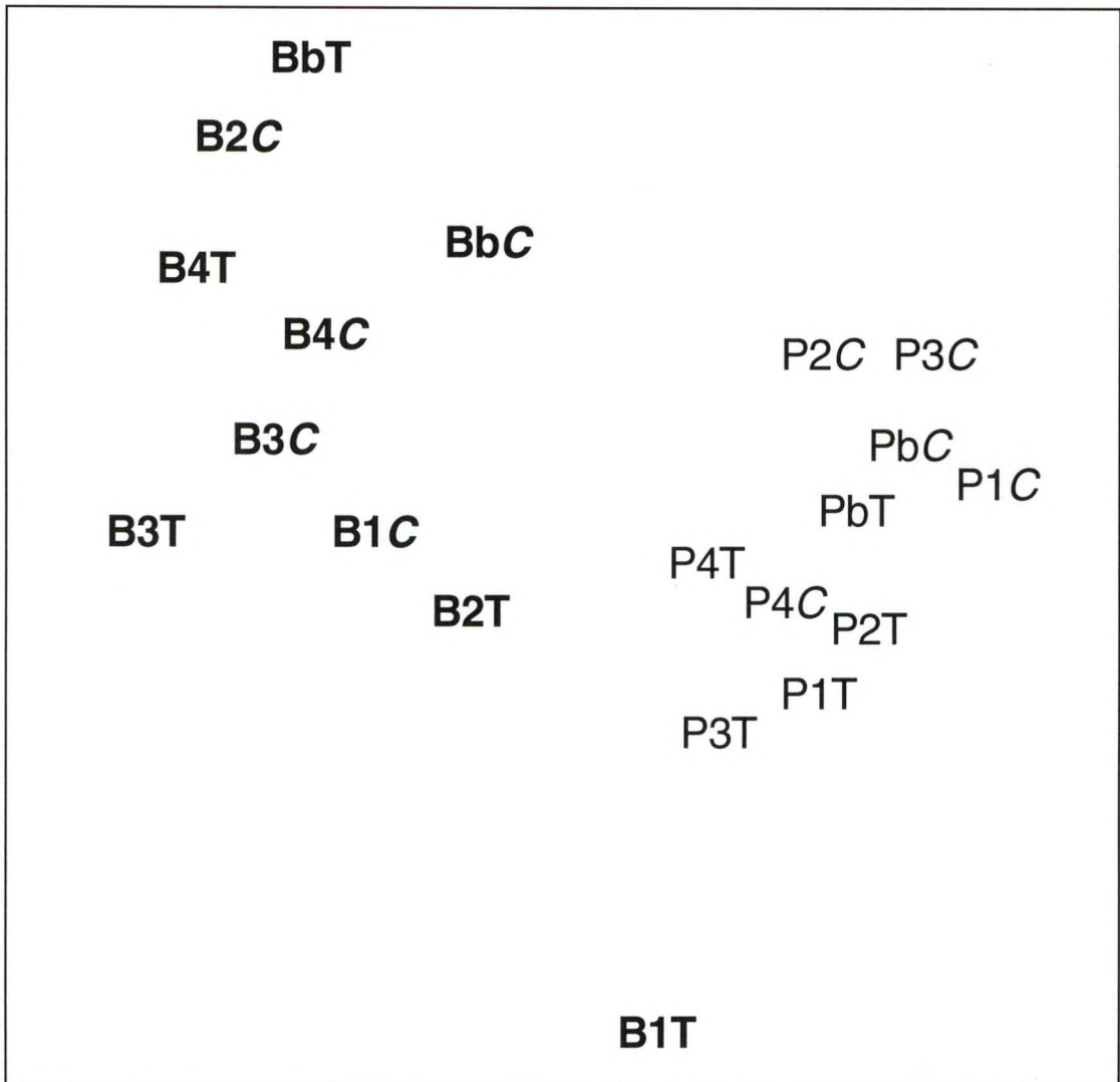
Fig. 3.6.14. MDS plot showing groupings based on stomach contents (stress value=0.14). Nomenclature as follows: XyZ - X = species ( B P. bernhardus , P P. prideaux ), y = days after fishing ( b = before, 1 = 1 day after etc.), Z = line ( C control, T treatment).
