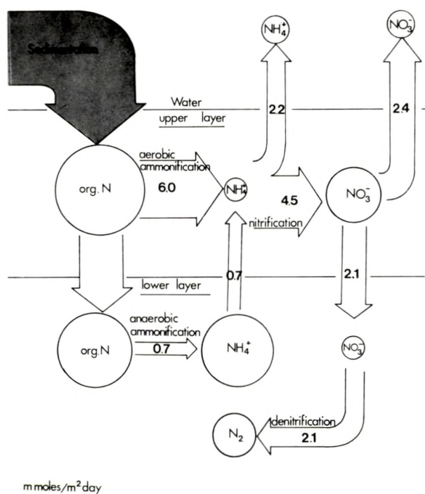
Fig 90 : Schematic representation of nitrogen transformations within the two layers of sediment and its fluxes across boundary between the two layers and sediment-water interface. (Vanderborght et al.1977).
