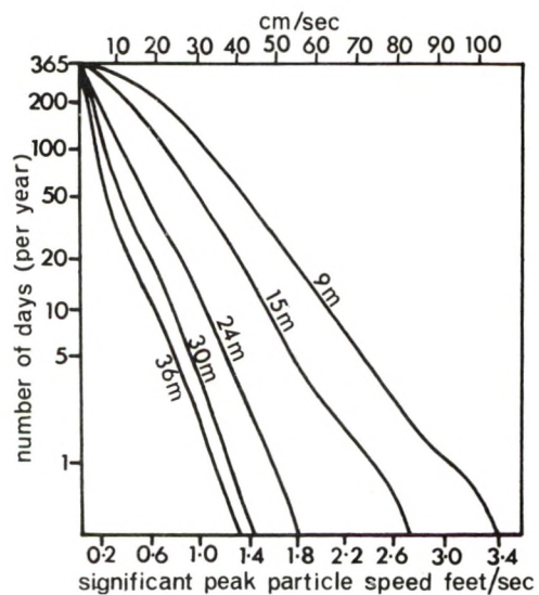
Figure85. The percentage of time during which water particle speeds near the sea floor exceed given values for five water depths. The graph is based on instrumental wave records at Smiths Knoll lightvessel, but can probably be used to indicate oscillatory current strength for much of the Southern Bight during moderate storms (after Draper 1967).
