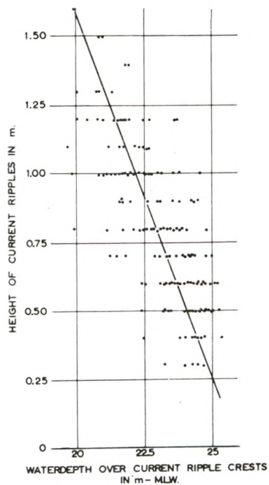
Fig.84.Variation of ripple height with water depth for ripples on side of sand waves.
