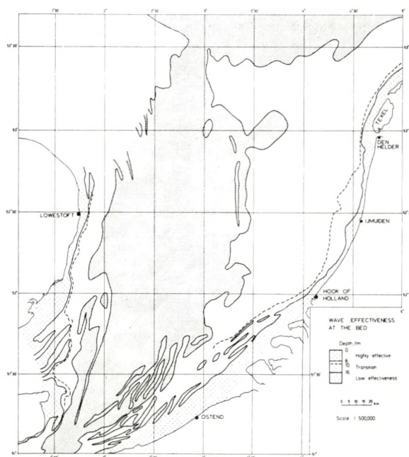
Fig. 86. Theoretical wave effectiveness at the bed from calculations based on the data of Draper (1967) by McCave (1971).
