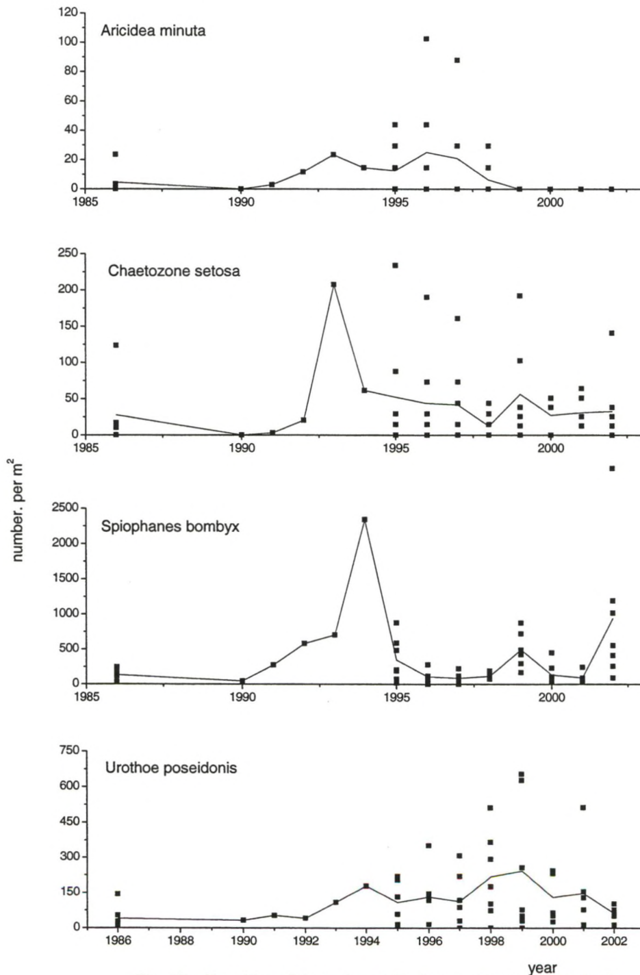
Fig. 13c: Densities of 4 species at the Dogger Bank (1986-2002)
