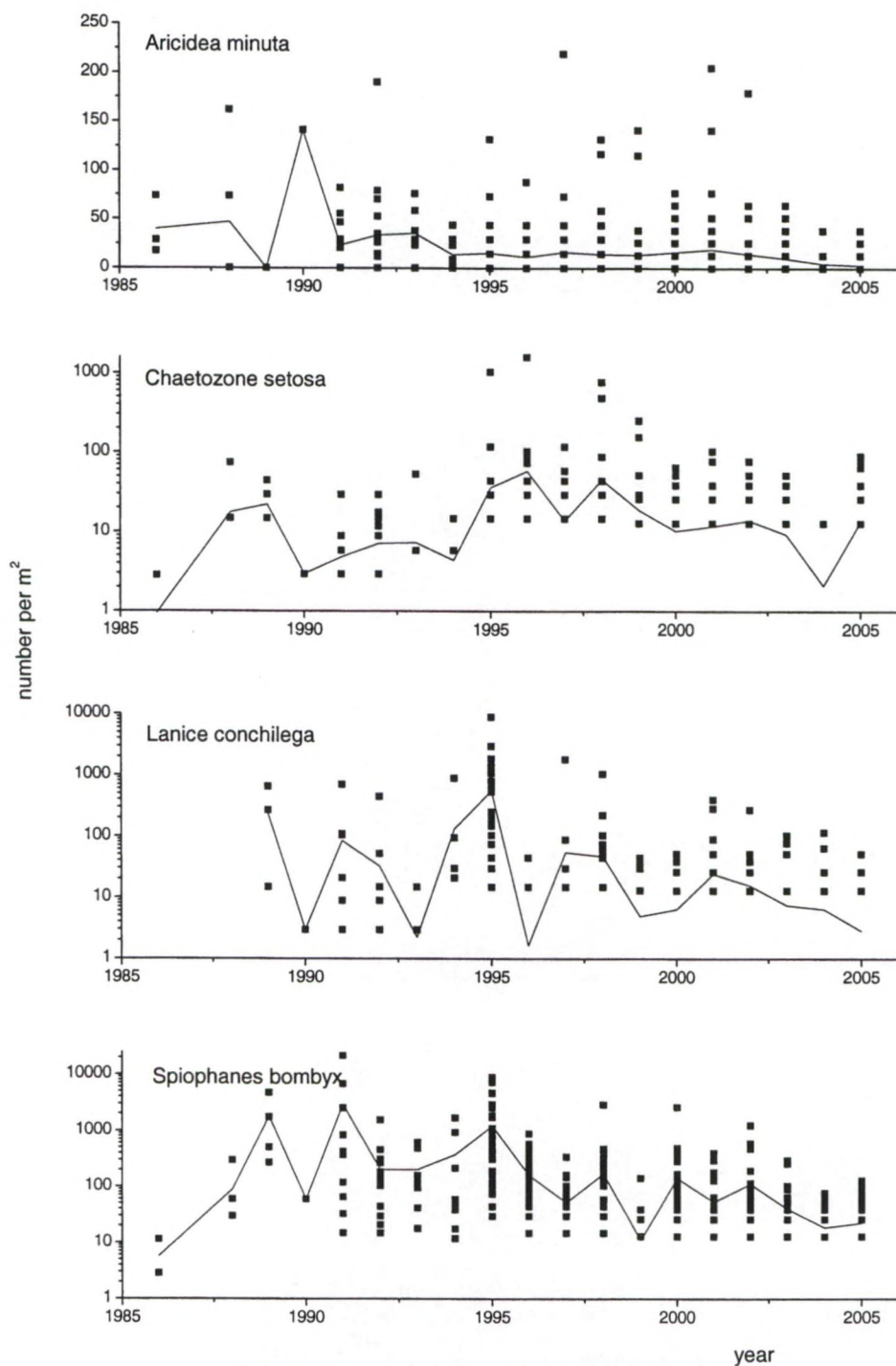
Fig. 15c: Densities of 4 species in the offshore area (1986-2005).
