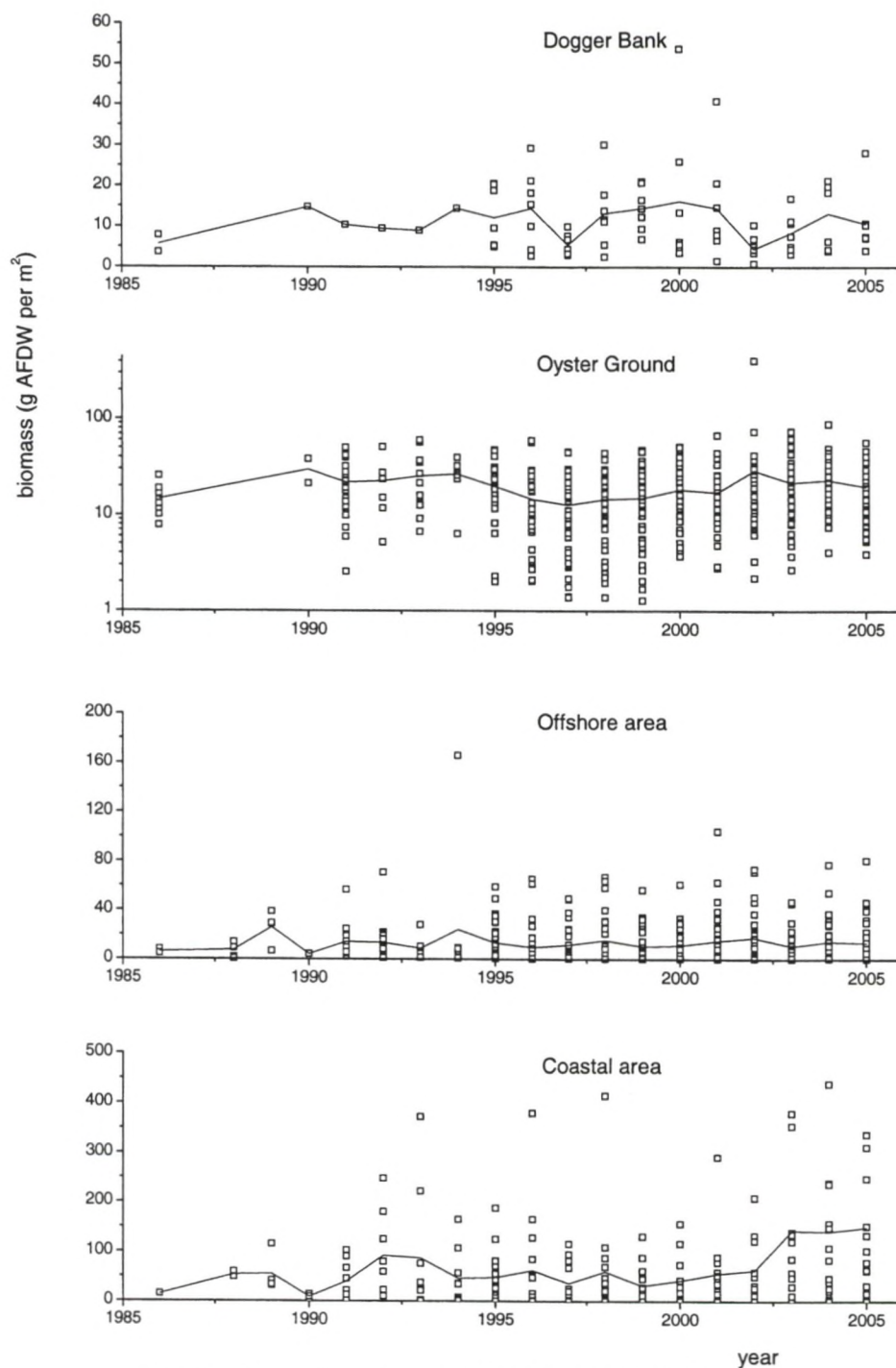
Fig. 12: Temporal patterns in biomass between 1986 and 2005.
