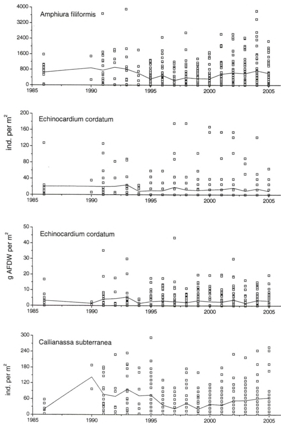
Fig. 14a: Densities (and biomass for E. cordatum ) of 3 species in the Oyster Ground (1986-2005).
