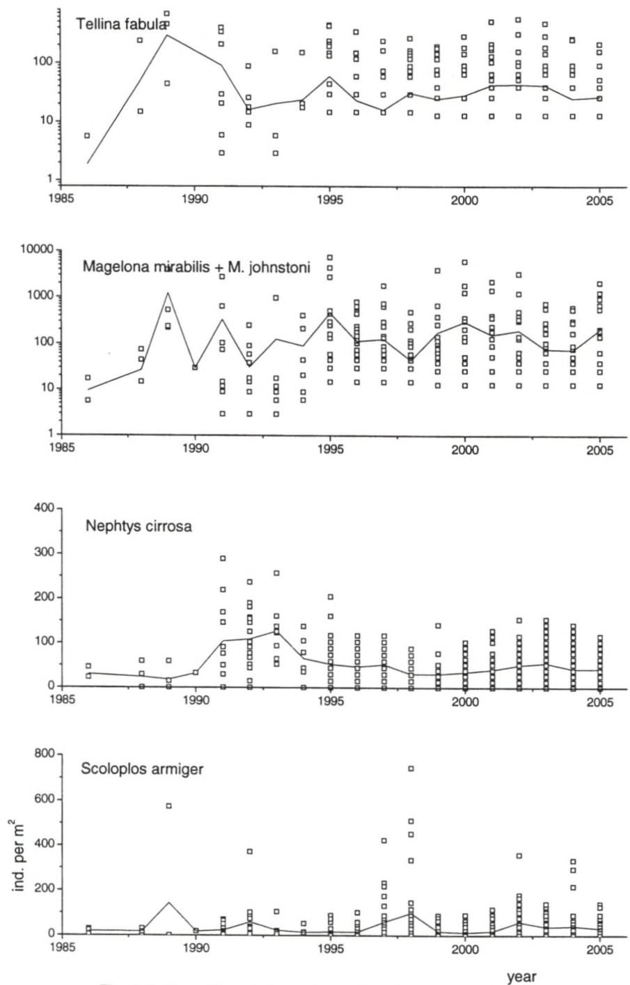
Fig. 15b: Densities of 4 species in the offshore area (1986-2005)
