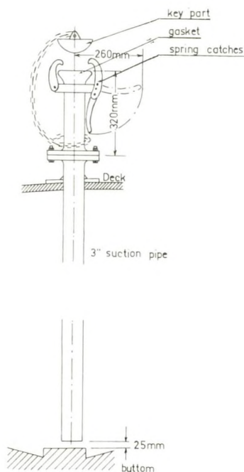
Fig. 6. Suction pipe for the fishing vessel.
