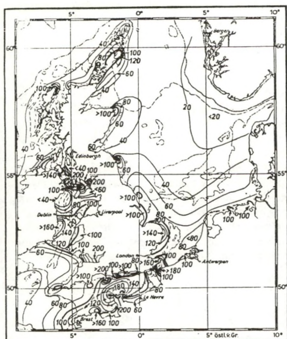
Fig. 5. Maximum tidal current velocity (surface, springtide) in \text{cm}\cdot\text{s}^{-1} (DIETRICH, 1950).
