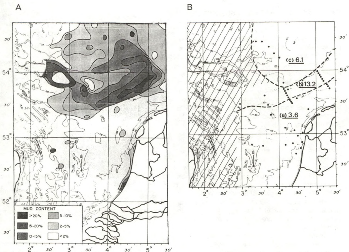
Fig. 55. Distribution of sediments according to mud content (<50 \mu\text{m} ), in the Southern Bight of the North Sea (A). Mean biomass (g AFDW \cdot\text{m}^{-2} ) of the benthic macrofauna in three different sectors (a), (b) and (c) in the same area (B). The dots are sample stations (CREUTZBERG et al. , 1984).
