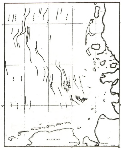
Fig. 17. Salinity fronts in the German Bight, 16–20.8.1979. Position of the frontal systems: —, S strongly increases towards the west; ---, S strongly decreases towards the west. (BECKER & PRAHM-RODENWALD, 1980)
