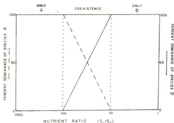
Fig. 47. Relative abundance of two phytoplankton species, A and B, plotted against the log of the ratio of limiting nutrients, S_1 and S_2 (PARSONS & HARRISON in: PARSONS et al. , 1984).
