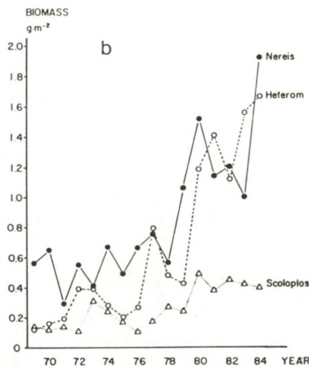
Fig. 45. Changes in total macrozoobenthos production (in \text{g AFDW} \cdot \text{m}^{-2} \cdot \text{yr}^{-1} ) in a tidal flat area in the western Wadden Sea. Estimates based on samples taken along 12 transects (open points) and in three squares (solid points) (a). Increasing standing stocks (in weight units) in three species of worms in the same area (b). (BEUKEMA, 1987 and BEUKEMA & CADEE, 1986).
