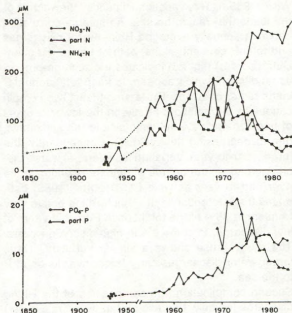
Fig. 27. Concentrations of \text{PO}_4^{3-} , particulate P, \text{NH}_4^+ , \text{NO}_3^- and particulate N (all in µM) in the river Rhine. Data before 1900 after CLARKE (1920). Data between 1928 and 1945 annual averages measured at Rhenen, the Netherlands, calculated after BIEMOND's reports "De Watervoorziening van Amsterdam", 1940 I, p. 210 and 1948 p. 110. Data after 1955, annual averages measured at Lobith (German–Dutch border) calculated from the yearbooks of the International Commission for protection of the Rhine against pollution. Values until 1978: VAN BENNEKOM & SALOMONS (1981); 1978 and later: (VAN BENNEKOM, pers. comm.)
