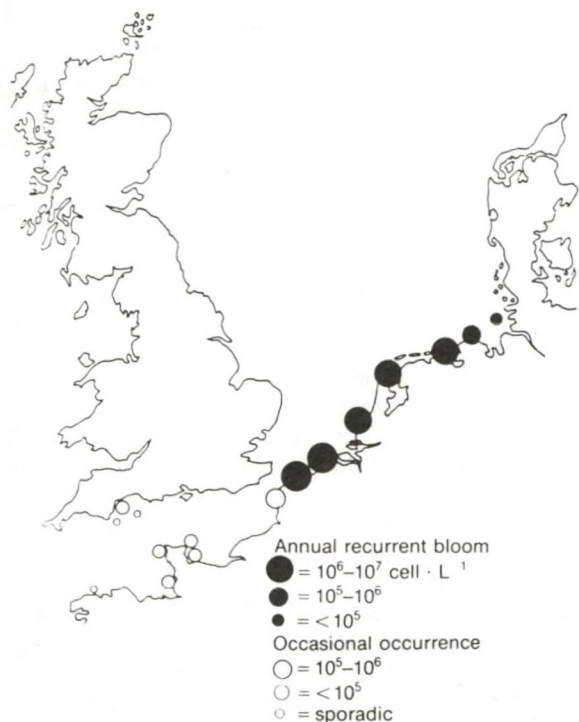
Fig. 51. Geographical distribution of Phaeocystis pouchetii . Maximum numbers are recorded at a few stations in the Channel and Southern Bight of the North Sea (LANCLOT et al. , 1987).
