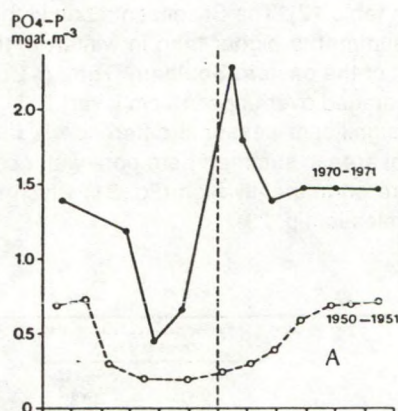
Fig. 33. Seasonal cycle of phosphate in the western Dutch Wadden Sea (Marsdiep tidal inlet area) in 1950–1951 and 1970–1971. After DE JONGE & POSTMA (1974). (POSTMA, 1982)
