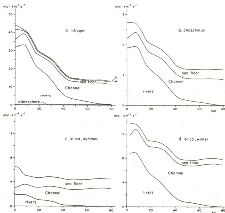
Fig. 23. Composition of nutrient inputs ( \text{mol} \cdot \text{km}^{-1} \cdot \text{s}^{-1} ) to Southern Bight waters off Holland as a function of offshore distance; river and English Channel inputs are flow rates at a section normal to the coast at IJmuiden (the increase in the river input from 0 to about 7 km offshore is related to the increase in water depth). Inputs from the sea floor (s, summer; w, winter) and from atmospheric deposition are the total inputs during the transit of the water over the study area (longshore length 120 km). (RUTGERS VAN DER LOEFF, 1980b).
