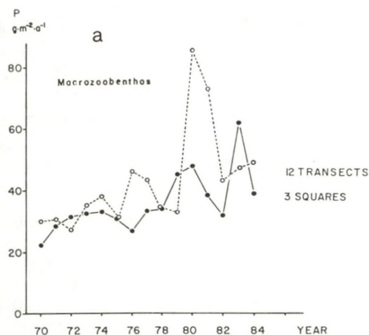
Fig. 45. Changes in total macrozoobenthos production (in \text{g AFDW} \cdot \text{m}^{-2} \cdot \text{yr}^{-1} ) in a tidal flat area in the western Wadden Sea. Estimates based on samples taken along 12 transects (open points) and in three squares (solid points) (a). Increasing standing stocks (in weight units) in three species of worms in the same area (b). (BEUKEMA, 1987 and BEUKEMA & CADEE, 1986).
