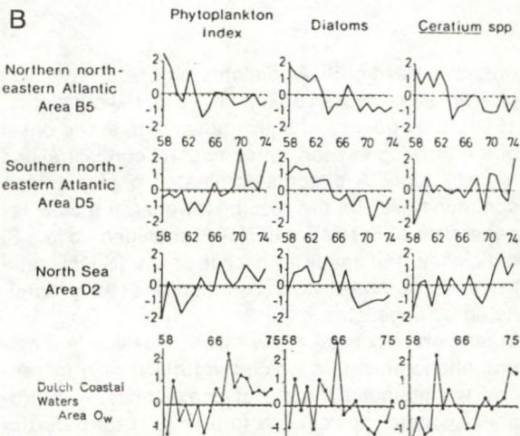
Fig. 49. Standard areas for Continuous Plankton Recorder Surveys; hatched area = area Ow (a) Annual mean abundance of phytoplankton in areas B5, D5, D2 and Ow (b) (after GIESKES & KRAAY, 1977b and REID, 1977).
