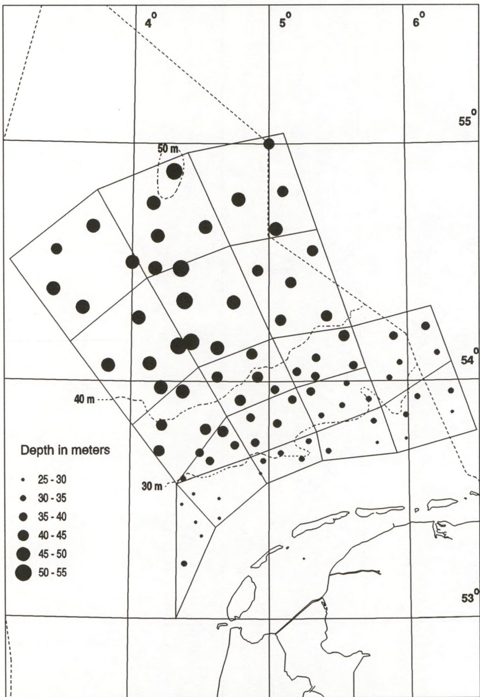
Fig. 4. Depth (m) recordings, uncorrected for differences due to the tidal cycle. Official 30, 40 and 50 m isobaths are indicated.
