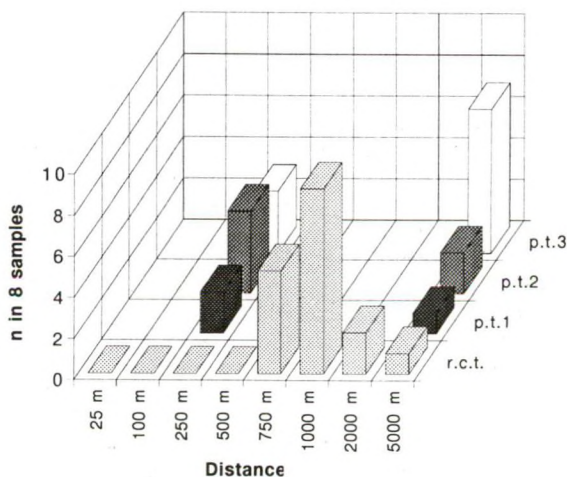
Fig. 9. Abundance of Echinocardium cordatum (specimens > 15 \text{ mm} ) around P6b.
