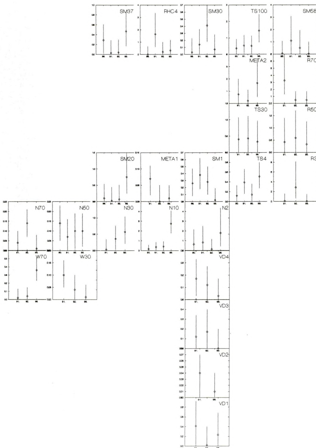
Fig. 5r. Comparison plots with the total biomass of the Miscellaneous species (g.AFDW./m²), for the period 1986 - 1993 (Note that only part of the stations were sampled prior to 1991). The 95% comparison limits are presented as bars; non overlapping bars denote a significant difference between the corresponding means.
