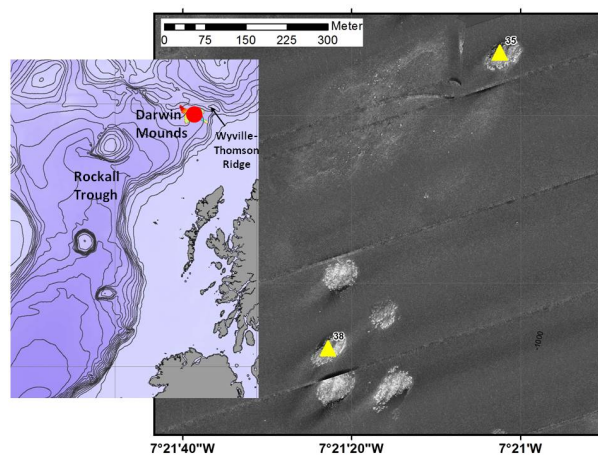
FIGURE 1. Sidescan sonar detail of the two Darwin Mounds cored during JC060. Left: location map of the Darwin Mound area
