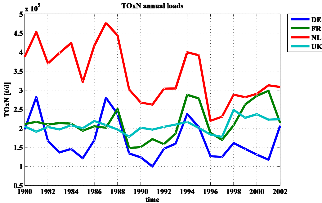
Figure 2.1. Available annual loads of TOxN ( \text{NO}_3 + \text{NO}_2 ) by country.
