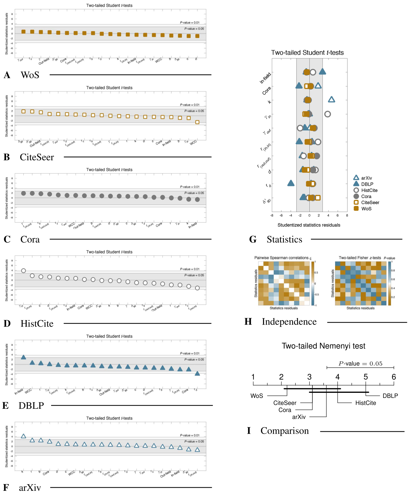
Figure 2 | Comparison of bibliographic databases through statistics of citation networks. Panels (A–F) show studentized statistics residuals of citation networks extracted from bibliographic databases. The residuals are listed in decreasing order, while the shaded regions are 95% and 99% confidence intervals of independent Student t -tests (labelled with respective P -values). Panel (G) shows the residuals of merely independent statistics, where the shaded region is 95% confidence interval. Panel (H) shows pairwise Spearman correlations of independent statistics listed in the same order as in panel (G) (left) and the P -values of the corresponding Fisher independence z -tests (right). Panel (I) shows the critical difference diagram of Nemenyi post-hoc test for the independent statistics. The diagram illustrates the overall ranking of the databases, where those connected by a thick line show no statistically significant inconsistencies at P -value = 0.05 (see Methods).
