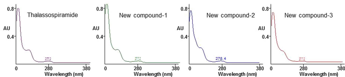
Figure 3 | Screening for strains with similar secondary metabolite profiles as Thalassospira sp. TrichSKD10 and the discovery of new thalassospiramide analogues. (a) UPLC comparison of T. sp. TrichSKD10 and MarineB0701 (classified as T. xiamenensis by ribotyping) found by searching our database. The potentially novel compounds are labeled with a star. (b) Comparison of UV absorptions of thalassospiramide and 3 new compounds. The maximum absorption wavelengths of 4 compounds were very similar.
