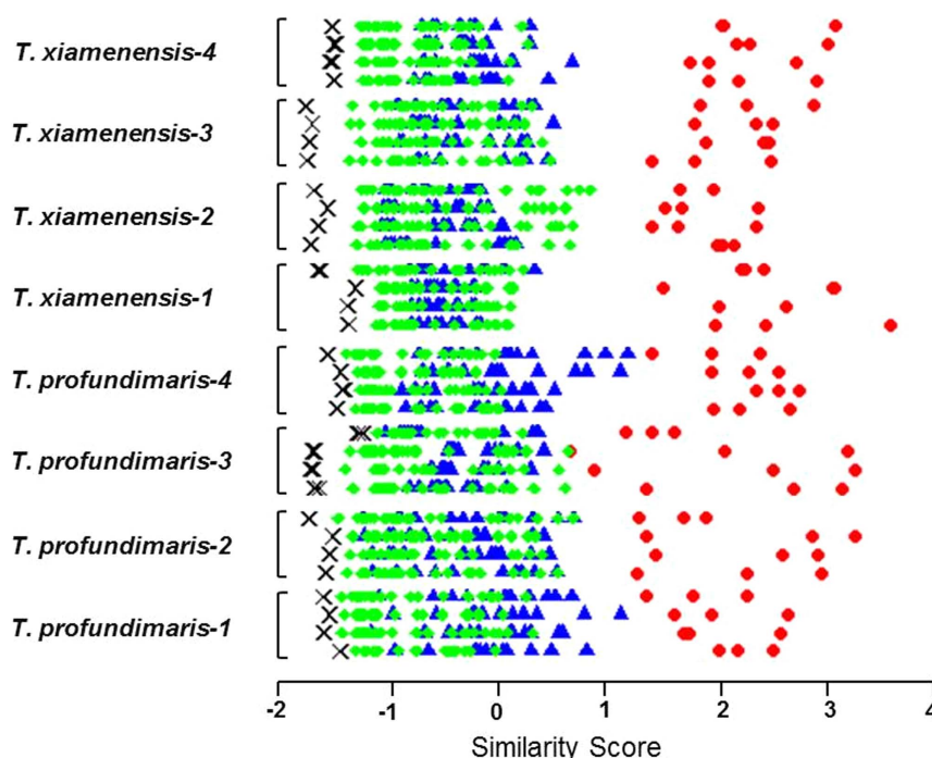
Figure 1 | Similarity of secondary metabolite profiles of Thalassospira strains at different taxonomic levels. A small test database was constructed using 8 Thalassospira strains (4 of T. xiamenensis and 4 of T. profundimaris ) and 1 Pseudovibrio denitrificans strain (as negative control). Four biological replicates of each Thalassospira strains were cultured, and its secondary metabolite profiles are searched against the test database. The similarity scores between each biological replicate and all possible answers were plotted as data points on a horizontal line with the following color code: biological replicates of the same strain (red), different Thalassospira strains in the same species (blue), different Thalassospira species in the same genus (green), and the P. denitrificans strain (black). The secondary metabolite profiles of the same strain show high biological reproducibility, and the secondary metabolite profile similarity approximately, but not always, correlates with taxonomical similarity. The profiles of strains differing at the genus level are sometimes more similar than those differing at the species level.
