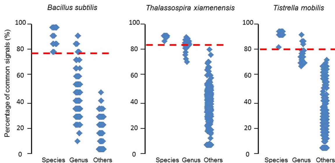
Figure 2 | Using common metabolite signals as a species-specific classification index. Common metabolite signals were extracted from 5 reference strains of each species ( B. subtilis , T. xiamenensis and T. mobilis ). Then each LC-MS profile in the database is searched for the presence of these signals, and the percentage found was plotted as a data point. The data points are sorted by taxonomical level: different strains of the same species (Species), different species of the same genus (Genus), and different genera (Others). The results indicate that the number of found "species-specific signals" correlates with the taxonomical similarity, and that one can potentially use these "species-specific signals" as a phenotypic classification index, e.g., percentages above the red line indicate strains from the same species.
