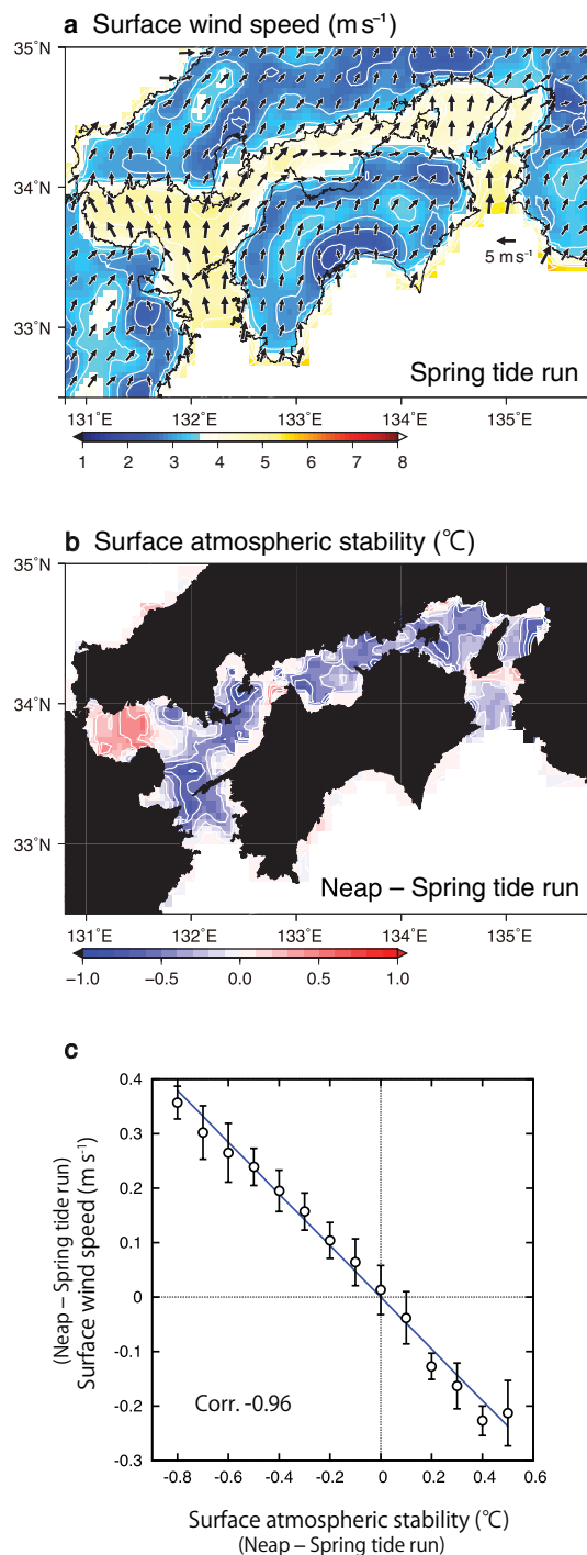
Figure 3. Modelled surface wind and surface atmospheric stability during summer. a–c, All values are averaged over summers (June–August) from 2003 to 2012. (a) Wind fields at 10 m in the spring tide run, and (b) surface atmospheric stability difference between spring and neap tide runs. Vectors indicate winds with scales shown in the middle right of the panel. See the text for the definition of the surface atmospheric stability in (c). Contour intervals are (a) 0.4 \text{ m s}^{-1} and (b) 0.2 ^{\circ}\text{C} . c, Scatter diagram between surface atmospheric stability versus wind speeds at 10-m height. The data are differences between neap and spring tide runs, and are averaged over summers (June–August) from 2003 to 2012 at each grid cell over the Seto Inland Sea. Open circles indicate mean wind-speed difference values within each bin of the stability difference with the interval of 0.1 ^{\circ}\text{C} , and the error bars represent \pm one standard deviation in each bin. The blue line indicates the regression line. The correlation coefficient is shown in the lower left corner of the panel (significant at P < 0.01 ). The correlation coefficient ( -0.96 ) was computed using data before the binned average ( n = 689 ). The Generic Mapping Tools were used to create the maps in (a) and (b). Gnuplot was used to create the graph in (c).
