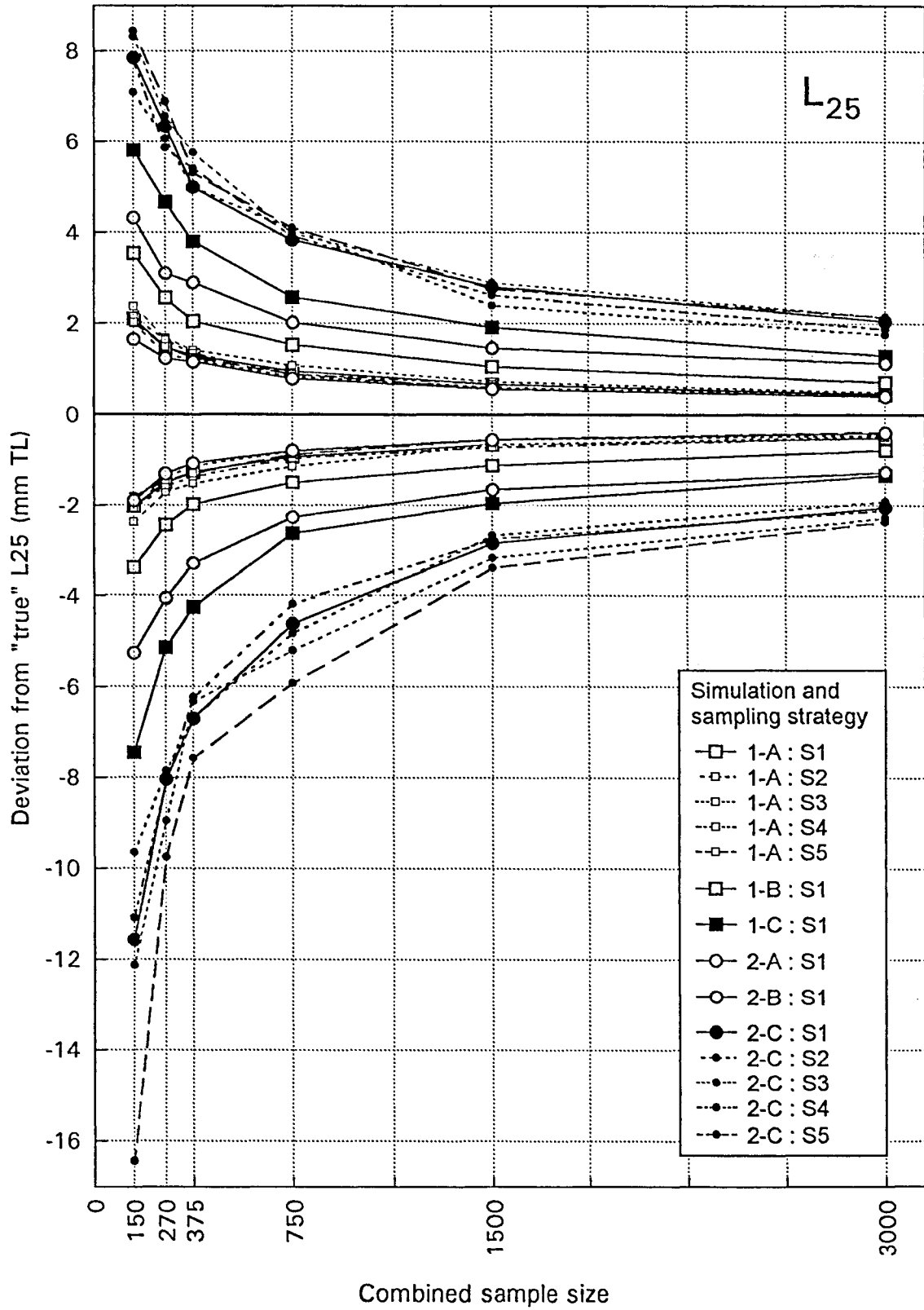
Figure 5 - 2.5 and 97.5 percentiles of the deviations of the "re-calculated" L25's, L50's and L75's from their "true" values for different sampling strategies and sample sizes
