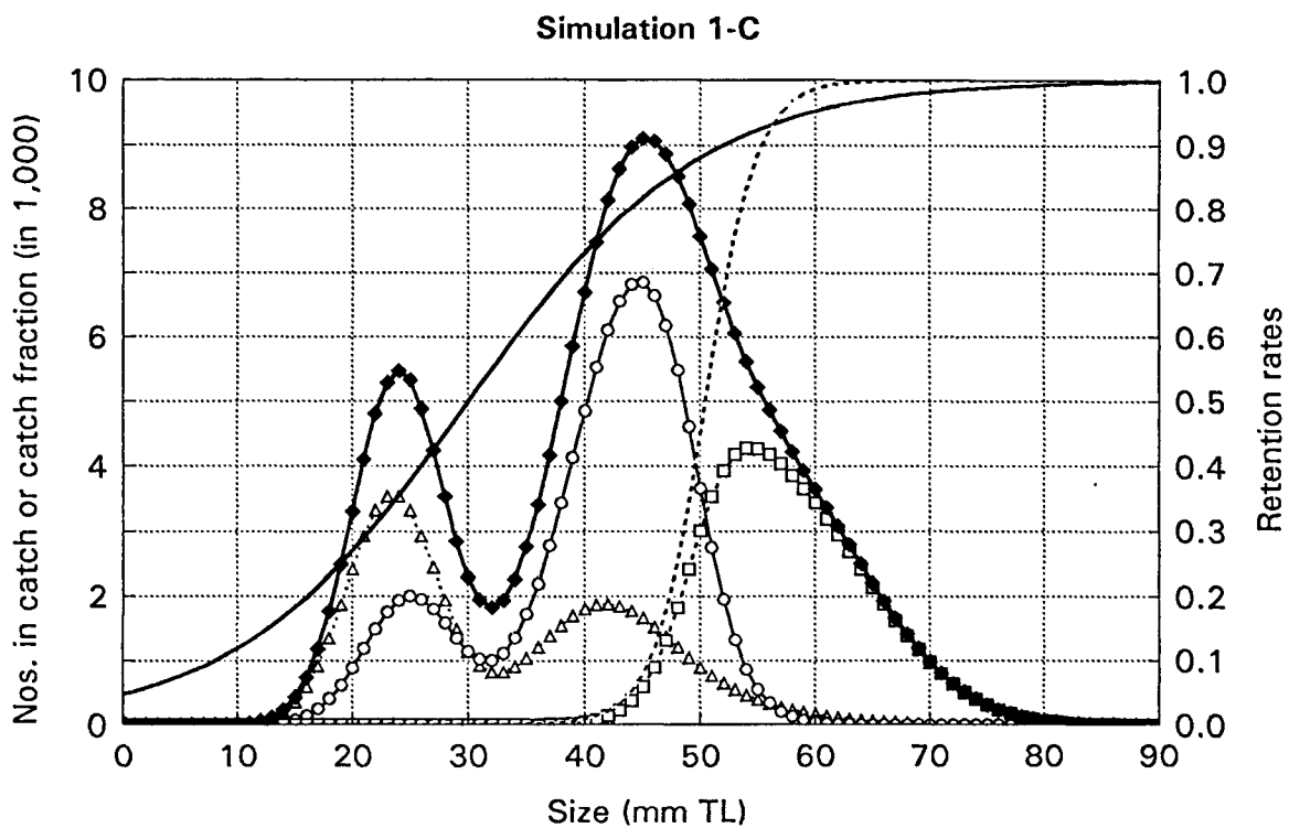
Figure 3 (continued) - Size compositions of the catch fractions used in simulations 1-A, 1-B and 1-C
