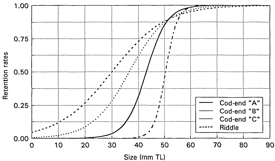
Figure 2 - Cod-end and shrimp riddle selection curves used in the simulations
