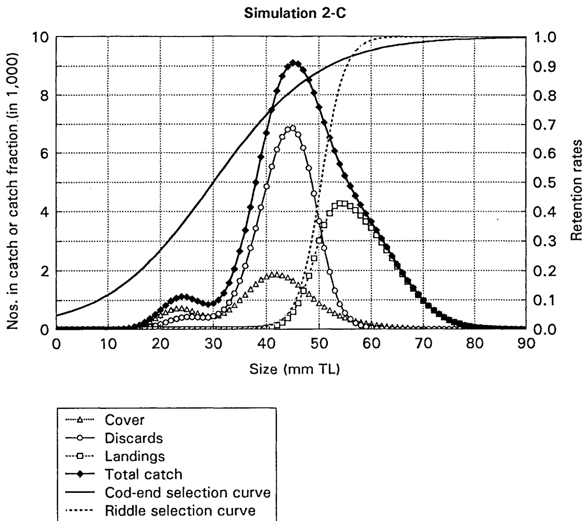
Figure 4 (continued) - Size compositions of the catch fractions used in simulations 2-A, 2-B and 2-C
