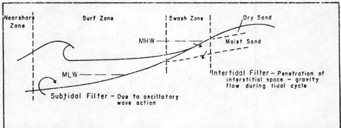
Figure 2. High-energy sand beach system (modified from Cox, 1976).
