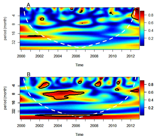
Figure 3. Squared coherence between Nino3.4, DMI and dengue incidence rate in Bangladesh (A: Nino3.4 and dengue, B: DMI and dengue). Statistical significance for coherence is determined by Monte Carlo simulations (300). Blue, low coherence; red, high coherence. The black lines show the areas where coherence is significantly high (95% confidence level). The cone of influence (white curve) indicates the region not influenced by edge effects.
