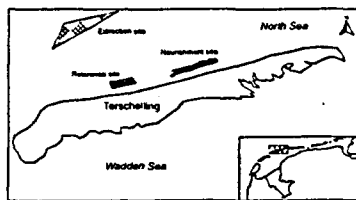
Figure 1. Location of the RIACON study sites off Terschelling
