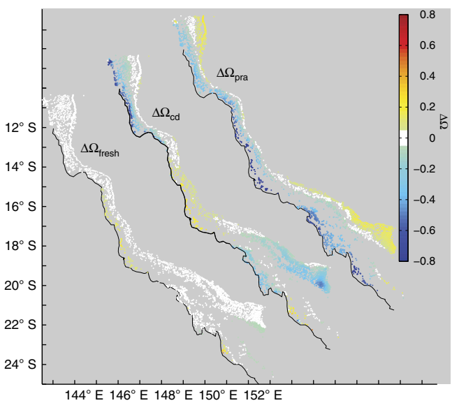
Figure 4 | Drivers of change in aragonite saturation. The changes are separated into the affect due to hydrological cycle ( \Delta\Omega_{\text{fresh}} ; left), net calcification ( \Delta\Omega_{\text{cd}} ; centre), and due to the combination of photosynthesis, respiration and air-sea exchange ( \Delta\Omega_{\text{pra}} ; right), average from daily September 2010–September 2012 values.
