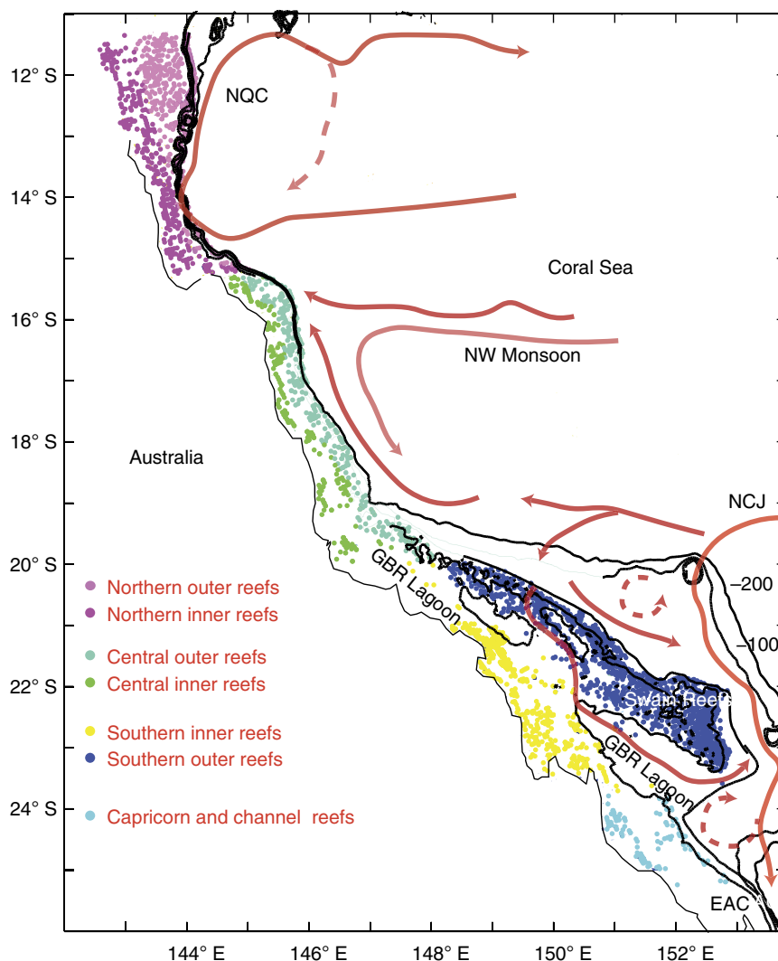
Figure 1 | Great Barrier Reef living coral distribution. Black lines show the 60, 100 and 200 m depth contours. Red lines show major surface currents. NQC: North Queensland Current; EAC: East Australian current; NCJ: North Caledonia Jet. Dashed orange lines show transient currents. The coloured dots show the individual reefs as identified by the Great Barrier Reef Marine Park Authority (GBRMPA) shelf features e-atlas separated into different geographical zones.
