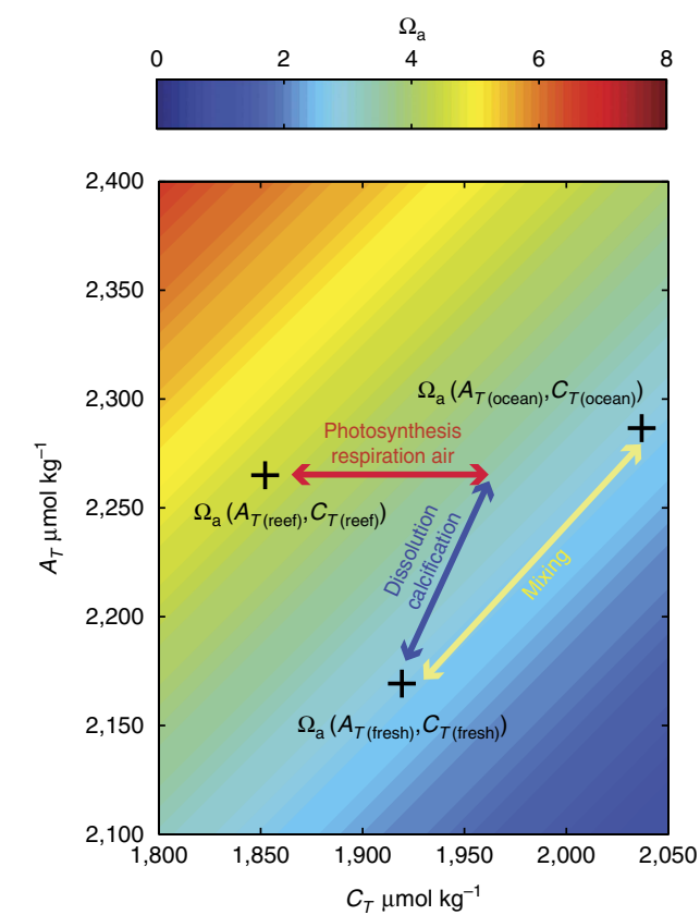
Figure 3 | Driver of aragonite saturation-state change schematic. The change from the open ocean value is separated into three drivers: (1) hydrological cycle calculated considering dilution/mixing associated with a change in salinity (yellow arrow); (2) Net calcification is calculated as a shift in alkalinity and dissolved inorganic carbon at a ratio of 2:1 (blue arrow); (3) net carbon uptake due photosynthesis, respiration and air-sea flux (red arrow). Based on these values, the change in aragonite saturation from the open-ocean state is calculated. Background shows aragonite saturation-state versus dissolved inorganic carbon, C_T , and total alkalinity, A_T , at a temperature of 25 °C and salinity of 35.
