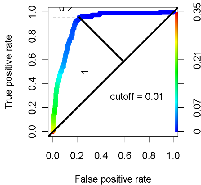
Figure B-93. Receiver operator characteristic (ROC) curve to determine optimal cutoff for binary habitat for Beaked whales guild during Summer season in East region.
