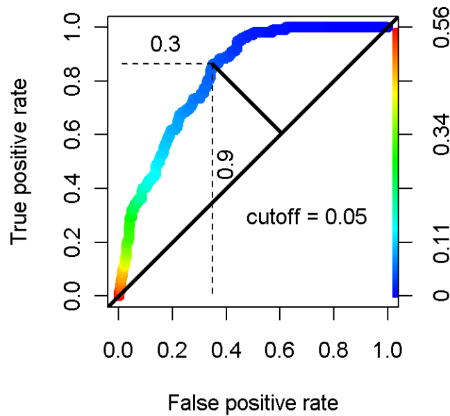
Figure B-75. Receiver operator characteristic (ROC) curve to determine optimal cutoff for binary habitat for Tursiops guild during Summer season in Gulf of Mexico region.
