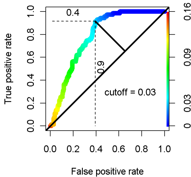
Figure B-33. Receiver operator characteristic (ROC) curve to determine optimal cutoff for binary habitat for Stenella attenuata guild during Summer season in Gulf of Mexico region.
