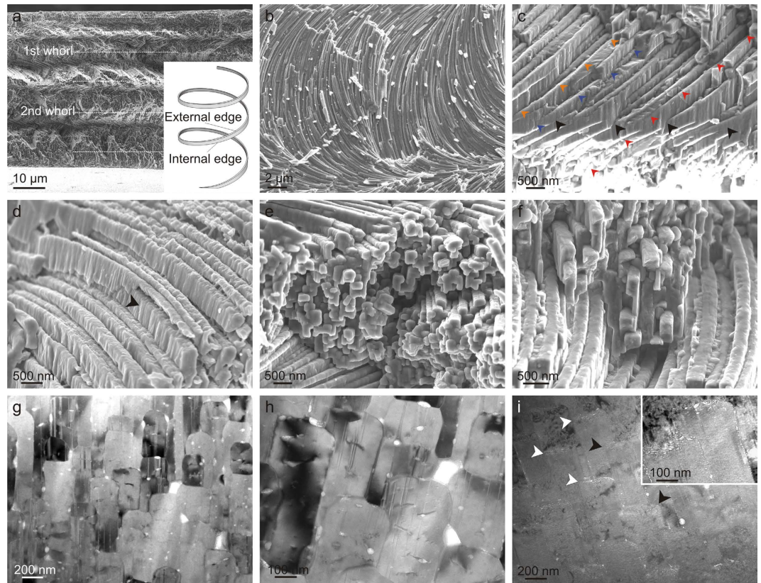
Figure 1. Fracture (SEM) and section (TEM) views of the AHFM of the Cavolinioidea. (a) Radial section of the shell of Cuvierina columnella . Horizontal broken lines are spaced at about half a turn. In this specimen, the helices complete some three turns. Note how the spacing between half turns (and, thus, the lead angle) increases towards the shell interior. The inset is a sketch of the ideal morphology of one such helical fibres. (b) Top view of a fracture through the shell of Cuvierina columnella , approximately parallel to the shell surface. The observed changes in orientation of fibres are caused by the unevenness of the fracture surface. (c) Fracture perpendicular to the surface of the shell of Cuvierina columnella , showing the interpenetration between fibres (black arrows). Colour arrows show the paths of three individual fibres (in different colours). (d) Etched fracture through the shell of Cavolinia longirostris . Etching permits a view of the complete process of crossing between two fibres; the lower fibre (arrow) crosses the upper fibre completely from right to left. (e,f) Transversely fractured fibres of Clio pyramidata (e) and Cuvierina urceolaris (f), showing the complex outlines caused by interlocking. (g) Transversal section of the fibres of Cuvierina columnella , exposing their interlocking cross-sections. The vertical thin lines within the fibres are twinning planes. (h) Detail of an area similar to (g). (i) Transversal section of the fibres of Cuvierina columnella . Fibres consistently show an external band (~150–200 nm thick) with an unusual density of white spots. The inset is a close-up of two such fibres. Arrows point to some examples. The external shell surface is to the top in (a) and (c) to (i).
