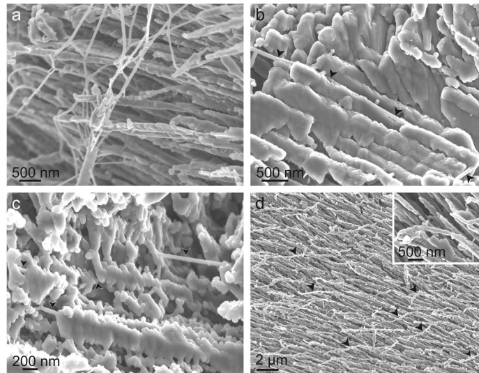
Figure 5. SEM views of semidecalcified fractures of the shells of the Cavolinioidae. (a) Cavolinia longirostris , showing the network of organic threads left after decalcification. (b) Cuvierina columnella . Long organic thread (>20 μm long, total length not shown) crossing a semidecalcified fibre through its external part (arrows). (c) Cuvierina columnella . Arrows point to organic fibres that have remained more or less in situ ; they consistently enter the corresponding fibres close to their external surfaces. (d) Specimen of Cavolinia longirostris in which the dissolution has not completely exposed the organic fibres, which are still surrounded by calcium carbonate granules. They appear as flexible thin extensions of the top parts of the mineral fibres, which have deflected leftwards during the treatment (some cases are indicated with arrows). The inset is a detail. (a,d) are views of the surfaces of the fibres looking towards the external shell surface. (b,c) are lateral views with the external shell surface to the top.
