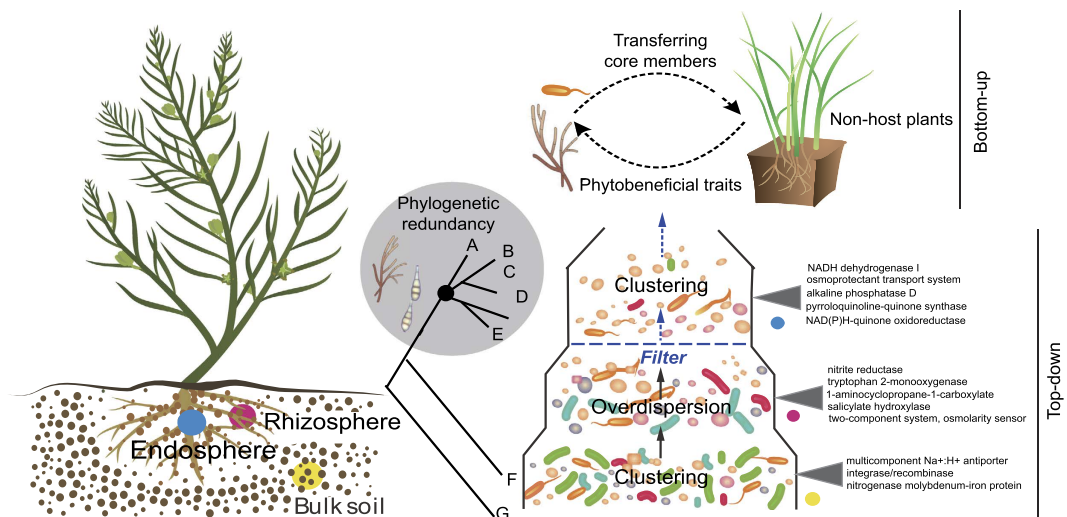
Figure 6. Conceptual illustration of the microbial community assembly and functional traits in the bulk soil (BS), rhizosphere soil (RS) and root endosphere (R). A rapid loss of diversity from soil (pedosphere) to the root endosphere (phytosphere) indicates the presence of a biotic filter at the root-soil interface (e.g., host genotype and root exudates). The dominant \alpha -proteobacteria and \gamma -proteobacteria communities in BS and R showed patterns of phylogenetical clustering, suggesting the microbial response to environmental extremes; there were over-dispersion trends in RS. In all habitats, a group of closely related MOTUs assigned to the same microbial lineages (at the genus level) indicated some degree of phylogenetic redundancy, a known buffering mechanism against stresses. The representative abundant functional genes predicted by PICRUST in each habitat were presented. These genes were often related to bacterial salinity tolerance and improved plant performance. Re-colonization and salt stress assays (a bottom-up approach) confirmed the extended phytobeneficial traits of some core culturable members on non-host plants.
