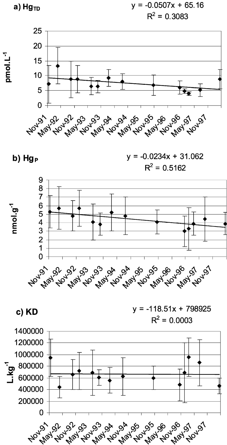
Fig. 3. Average concentrations and standard deviations of (a) total dissolved Hg (Hg TD ); (b) particulate Hg (Hg P ); and (c) the distribution coefficient of Hg (K D ) in the Scheldt estuary measured in the different surveys between 1991 and 1998.
