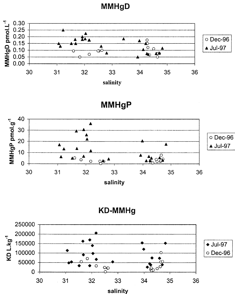
Fig. 8. Dissolved methylmercury (MMHg D ) and particulate methylmercury (MMHg P ) concentrations and their distribution coefficient ( K_D MMHg) vs. salinity in the Belgian coastal zone.
