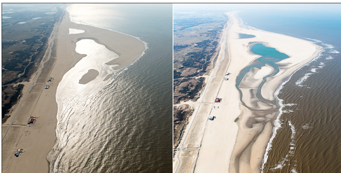
Figure 5 Southward looking aerial photograph of the Sand Engine at high water ( left ) and at low water ( right ) (spring 2013). Pictures courtesy of Rijkswaterstaat/Joop van Houdt.
