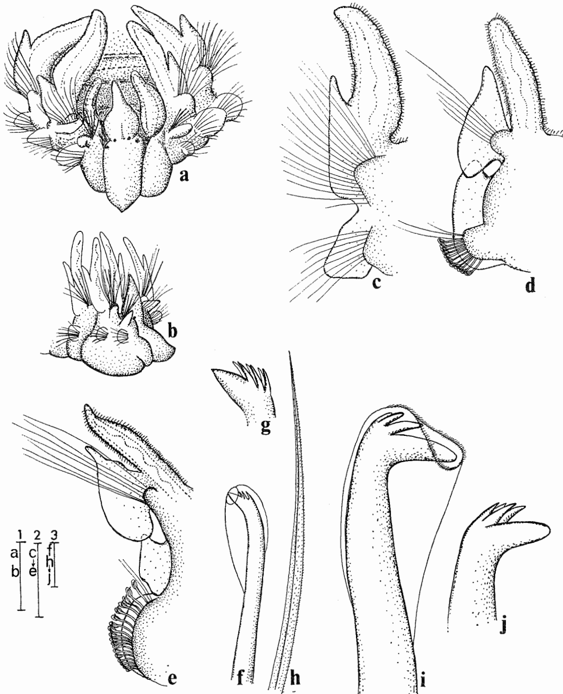
Figure 6— Scolelepis precirriseta sp. nov.—a, anterior end, dorsal view; b, anterior end, lateral view; c, right setiger 10, anterior view; d, right setiger 29, anterior view; e, right setiger 39, anterior view; f, multidentate hooded hook, lateral view; g, same, enlarged, hood omitted [not to scale]; h, superior capillary notoseta— Scolelepis sp.—i, hexadentate hooded hook, lateral view; j, hexadentate hooded hook, without hood showing arrangement of teeth, frontolateral view. [Scale 1 = 100 \mu m; 2 = 300 \mu m; 3 = 20 \mu m]
