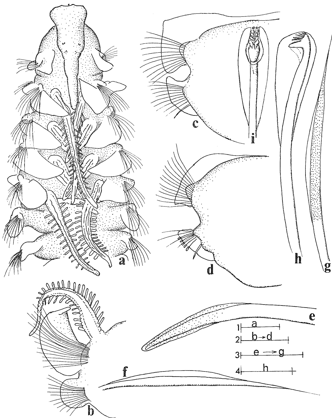
Figure 21— Prionospio queenslandica sp. nov.—a, anterior end, dorsal view; b, right setiger 5, anterior view; c, right setiger 12, anterior view; d, right setiger 20, anterior view; e, sabre seta; f, smooth capillary notoseta from setiger 5; g, granulated capillary notoseta from setiger 5; h, hooded hook, lateral view; i, same, frontal view. [Scale 1 = 200 \mu m; 2 = 300 \mu m; 3 = 50 \mu m; 4 = 20 \mu m; 5 = 10 \mu m]
