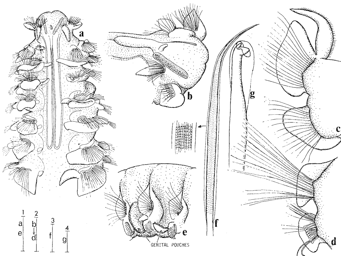
Figure 18— Laonice bassensis sp. nov.—a, anterior end, dorsal view; b, prostomium, antero-lateral view; c, right setiger 8, anterior view; d, right setiger 41, anterior view; e, genital pouches from about setiger 50, lateral view; f, anterior capillary seta [inset, detail of shaft, not to scale]; g, bidentate hooded hook. [Scale 1 = 200 \mu m; 2 = 50 \mu m; 3 = 50 \mu m; 4 = 20 \mu m]
