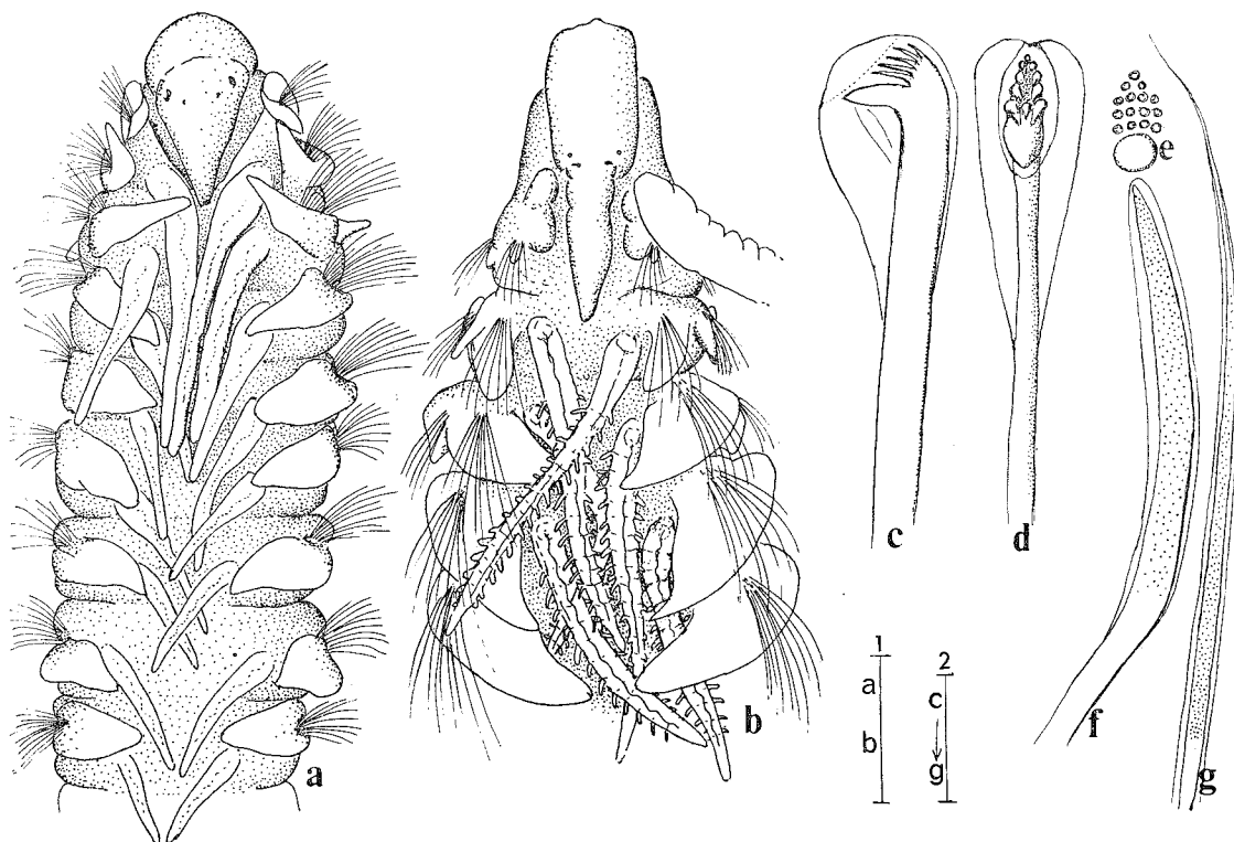
Figure 25— Prionospio cirrifera Wirén—a, anterior end, dorsal view— Prionospio aucklandica Augener—b, anterior end, dorsal view; c, hooded hook, lateral view; d, same frontal view; e, diagram of hooded hook tooth pattern at maximal development of secondary teeth; f, sabre seta; g, anterior capillary notoseta. [Scale 1 = 200 \mu m; 2 = 20 \mu m]
