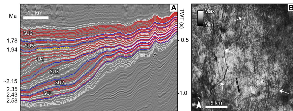
Fig. 2. Clinoform geometry, chronology, and iceberg scours. (A) Lines show the semiautomatically picked reflectors from the 3D seismic data. Blue lines show the seismic horizons that are used as a dating control and that define the six seismic units (see Methods and fig. S6). The red horizons are those with iceberg scours present, and the white horizons are those where glacial landforms have not been identified. The seismic line location is shown in Fig. 1C. The yellow dotted line shows the stratigraphic location of the surface mapped and displayed in (B). Mapping from picked reflectors/surfaces provides more robust chronological and depth/TWT (two-way travel time) control than mapping from time slices (22) (horizontal planes of equal TWT). (B) Surface created from the 3D seismic with the root mean square amplitude attribute displayed. White arrows show examples of curvilinear iceberg scours that were mapped on this surface. MegaSurvey 3D seismic data courtesy of PGS.
